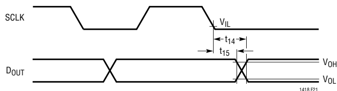
Figure 21. SCLK to \text{D}_{\text{OUT}} Delay
