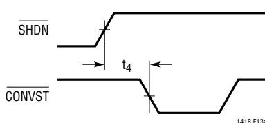
Figure 13a. SHDN to \overline{CONVST} Wake-Up Timing
