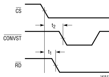
Figure 14. \overline{CS} to \overline{CONVST} Set-Up Timing
