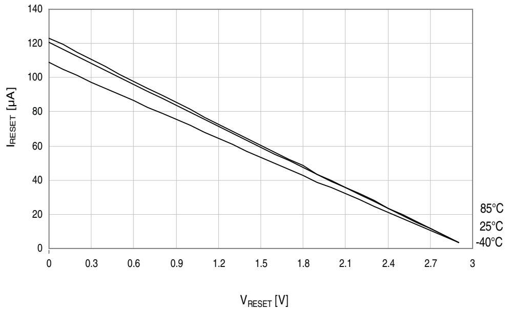
Figure 37-54. Reset pin pull-up resistor current vs. reset pin voltage. V_{CC} = 3.3V .
