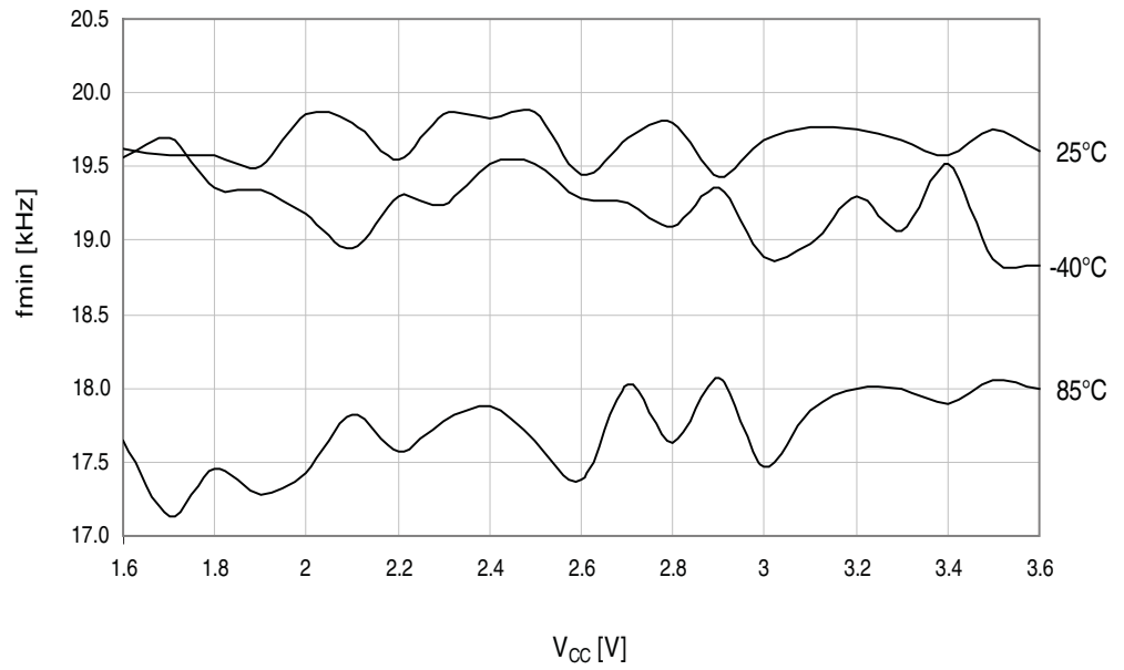
Figure 37-75. Maximum PDI frequency vs. V_{CC} .
