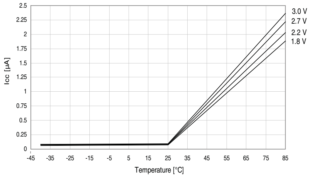
Figure 37-10. Power-down mode supply current vs. Temperature. All functions disabled.
