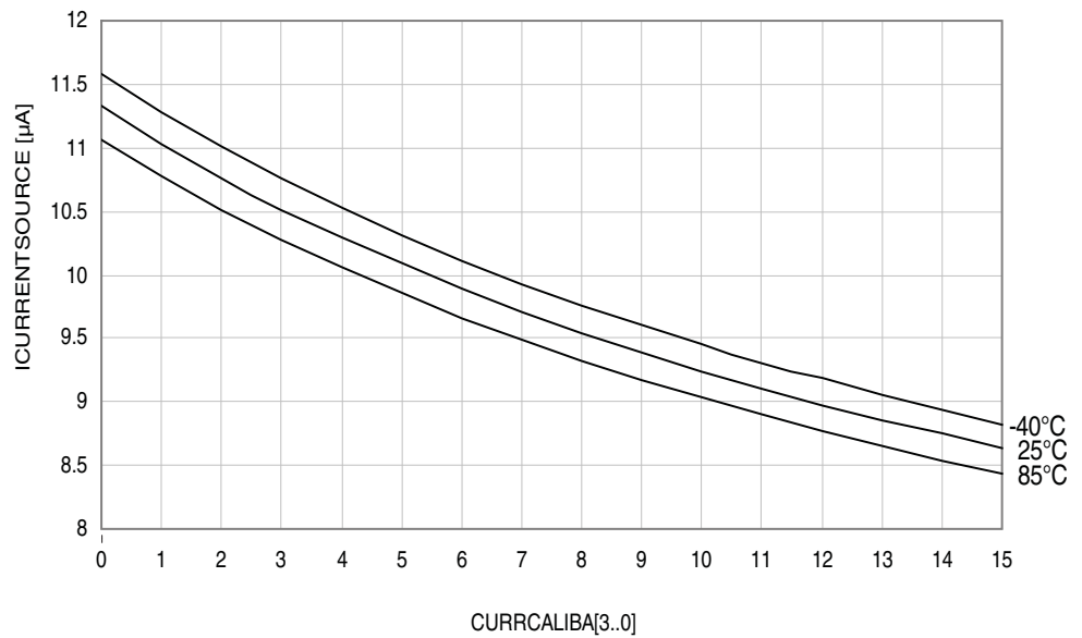
Figure 37-44. Analog comparator current source vs. Calibration. V_{CC} = 3.0V , double mode.
