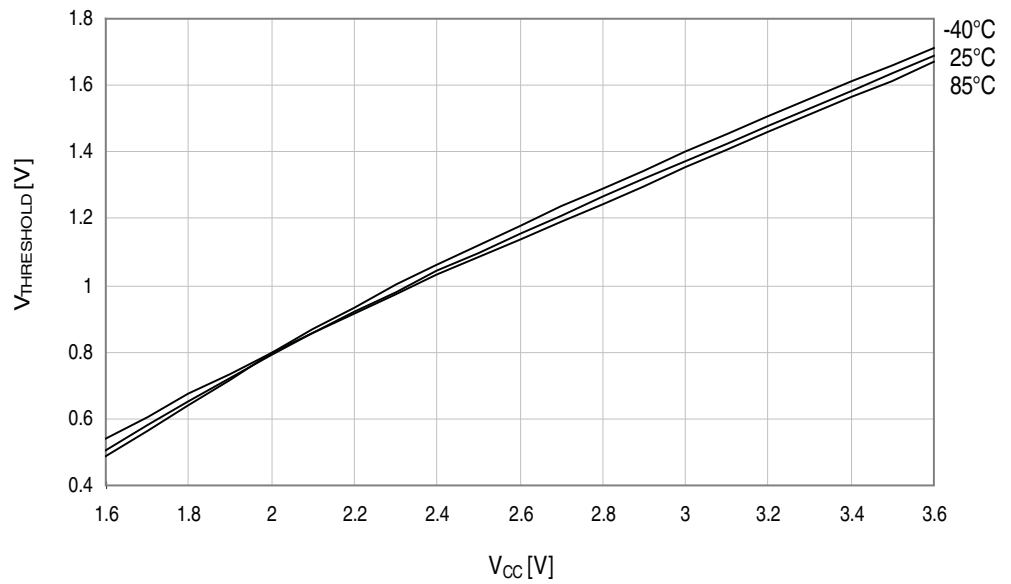
Figure 37-56. Reset pin input threshold voltage vs. V_{CC} .
