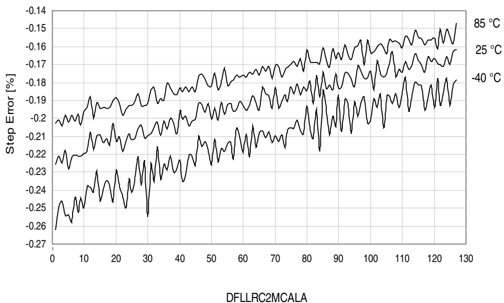
Figure 37-64. 2MHz internal oscillator CALB calibration step size.
