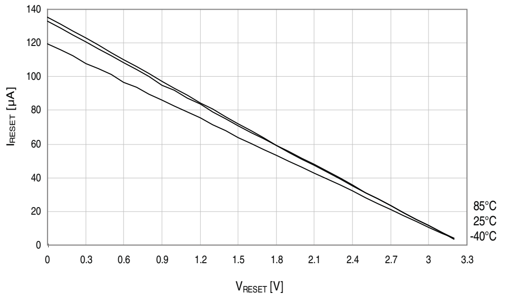
Figure 37-54. Reset pin pull-up resistor current vs. reset pin voltage. V_{CC} = 3.3V .
