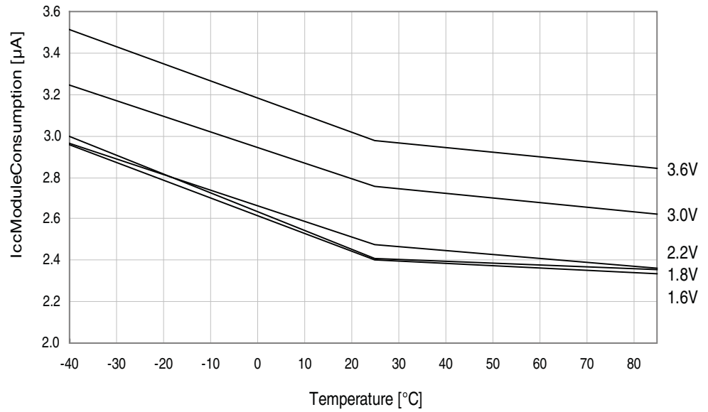
Figure 37-83. Psave vs. Temperature
