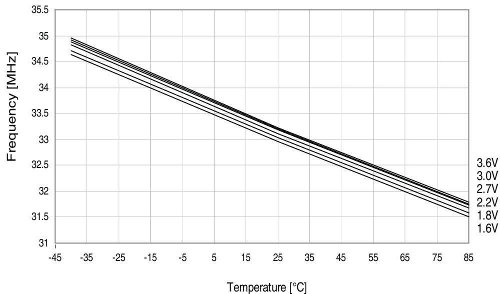
Figure 37-66. 32MHz internal oscillator frequency vs. temperature. DPLL enabled, from the 32.768kHz internal oscillator.
