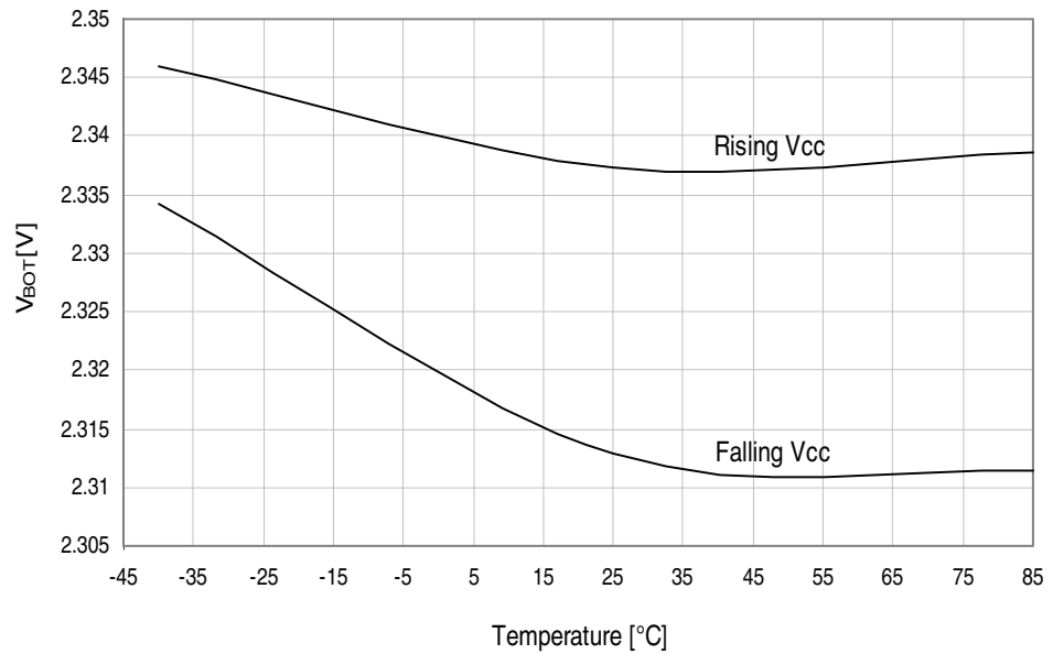
Figure 37-50. BOD thresholds vs. temperature.
