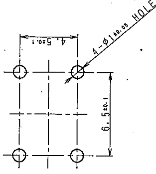
P.C. BOARD MOUNTING HOLE DIMENSIONS (WHEN VIEWED FROM SWITCH MOUNTING FACE)
