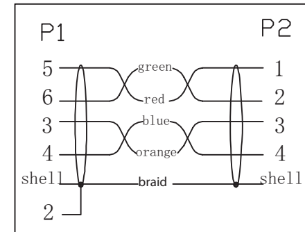
Wire Assignments
