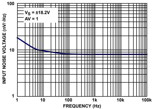
FIGURE 57. CHARACTERIZED INPUT NOISE VOLTAGE
