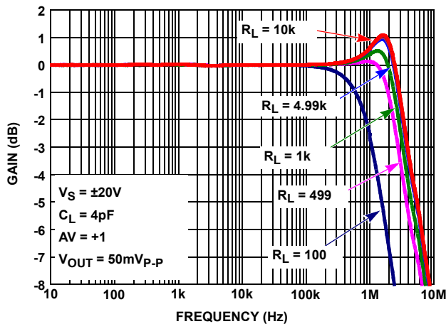
FIGURE 61. CHARACTERIZED CLOSED LOOP GAIN vs R_L
