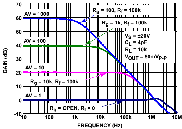
FIGURE 59. CHARACTERIZED CLOSED LOOP GAIN vs FREQUENCY
