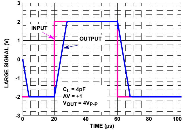
FIGURE 64. SIMULATED LARGE SIGNAL 10V STEP RESPONSE
