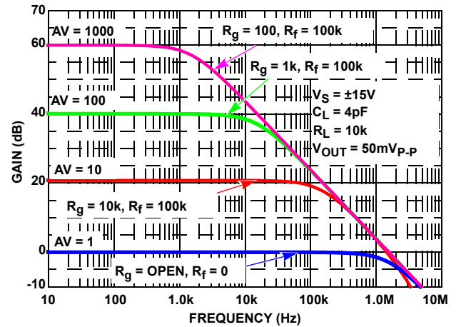
FIGURE 60. SIMULATED CLOSED LOOP GAIN vs FREQUENCY
