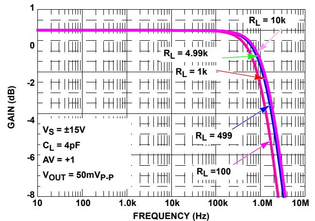
FIGURE 62. SIMULATED CLOSED LOOP GAIN vs R_L
