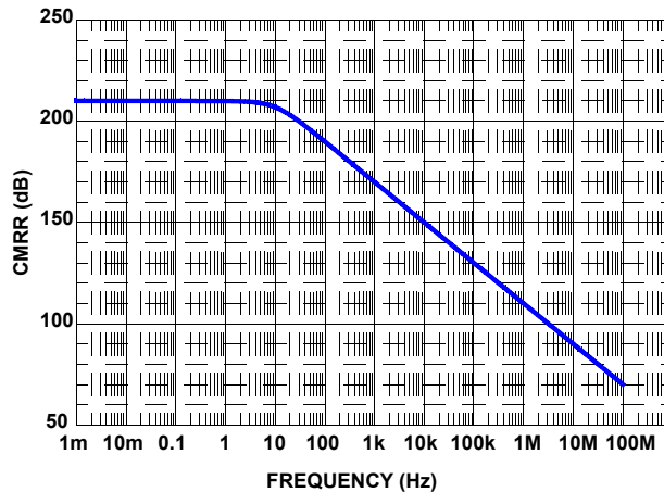
FIGURE 67. SIMULATED CMRR vs FREQUENCY
