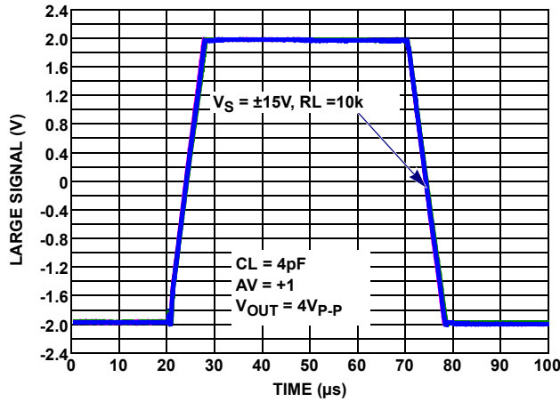
FIGURE 63. CHARACTERIZED LARGE SIGNAL TRANSIENT RESPONSE vs R_L V_S = \pm 15V
