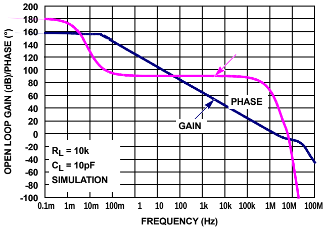
FIGURE 65. SIMULATED OPEN-LOOP GAIN, PHASE vs FREQUENCY
