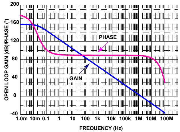
FIGURE 66. SIMULATED OPEN-LOOP GAIN, PHASE vs FREQUENCY
