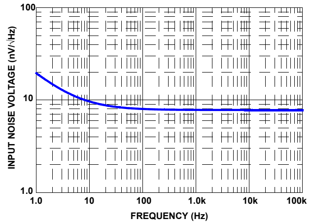
FIGURE 58. SIMULATED INPUT NOISE VOLTAGE
