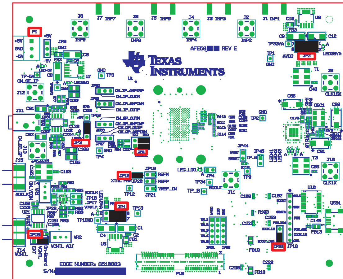
Figure 1. AFE5808/08AEVM Basic Configuration
