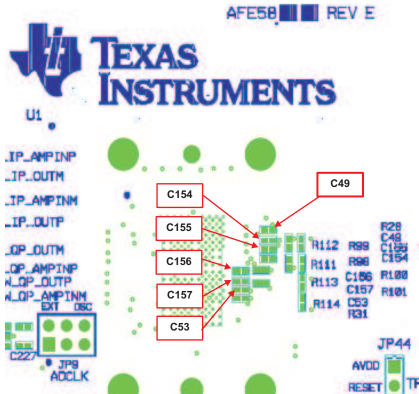
Figure 7. Relevant Capacitors for CW Mode, Top Side
