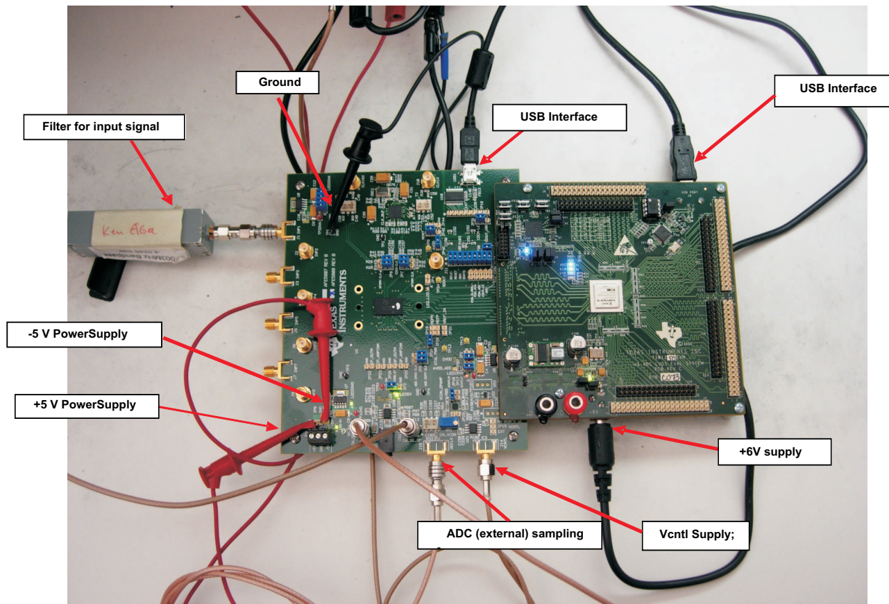
Figure 2. HW Setup With Connection Between TSW1250EVM and AFE5808/08A
