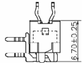
Mating Height Draw.
