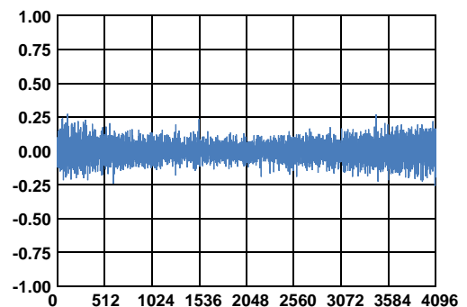
FIGURE 2. DIFFERENTIAL LINEARITY ERROR vs CODE
