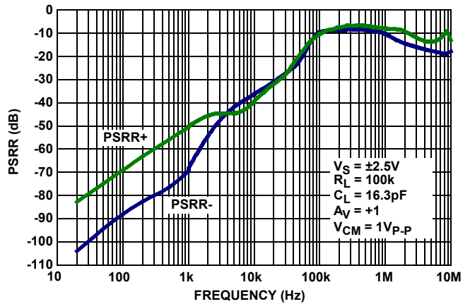
FIGURE 22. PSRR vs FREQUENCY, V_S = \pm 2.5\text{V}
