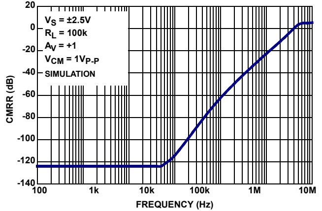
FIGURE 20. CMRR vs FREQUENCY, V_S = \pm 2.5\text{V}
