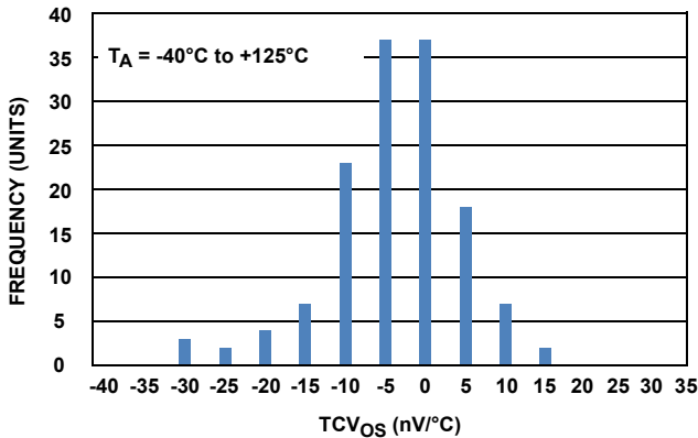
FIGURE 34. TCV_{OS} HISTOGRAM
