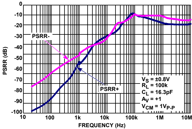
FIGURE 21. PSRR vs FREQUENCY, V_S = \pm 0.8\text{V}
