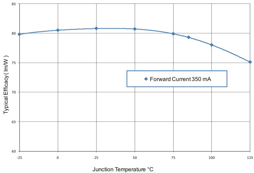
Figure 15. LXM8-PW27 and LXM8-PW30 emitters efficacy versus junction temperature.
