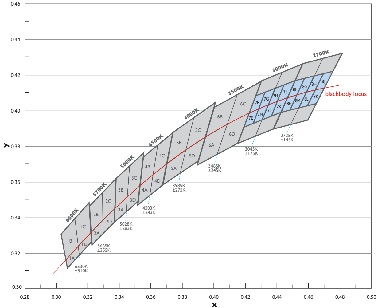
Figure 26. LUXEON Rebel ANSI I/I 6 th micro bin structure.
