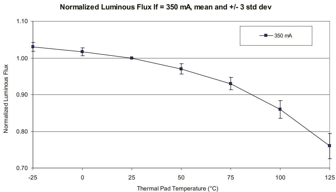
Figure 14. Relative light output vs. thermal pad temperature.
