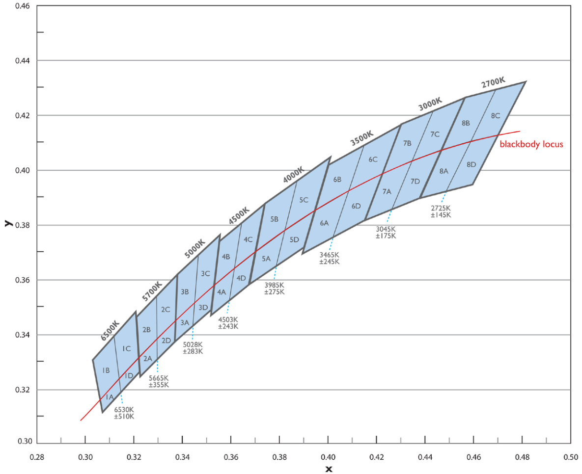
Figure 27. LUXEON Rebel ANSI I/4th quadrant bin structure.
