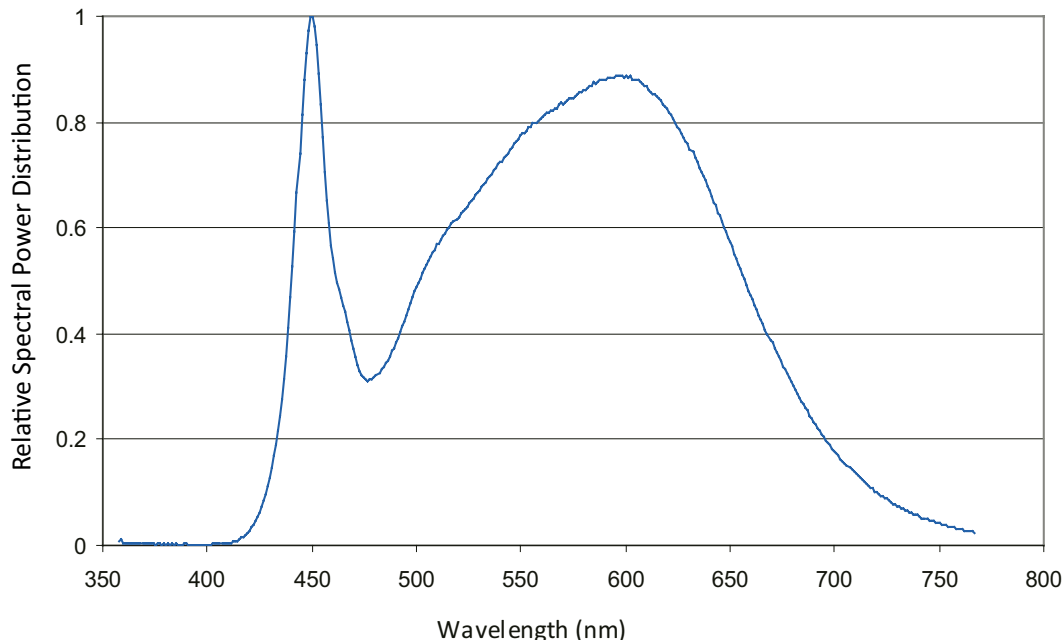
Figure 10. Color spectrum of LXM3-PW51 emitter, integrated measurement.
