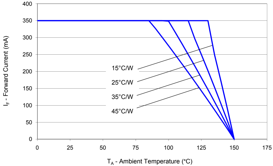
Figure 18. Maximum forward current vs. ambient temperature, based on T_{JMAX} = 150^{\circ}C .
