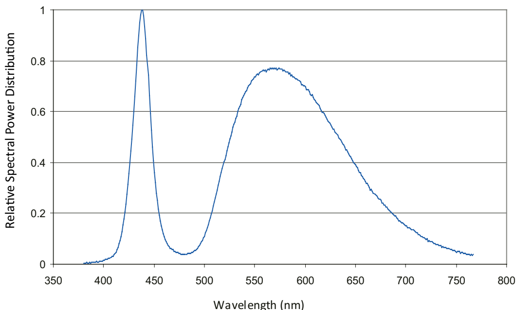
Figure 11. Color spectrum of LXML-PW51 emitter, integrated measurement.
