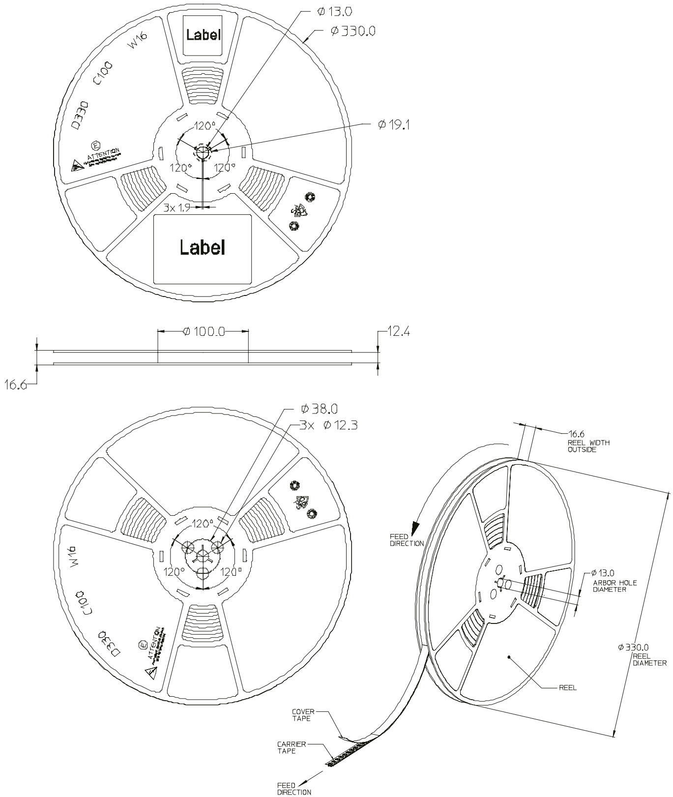
Figure 25. Emitter reel packaging.
