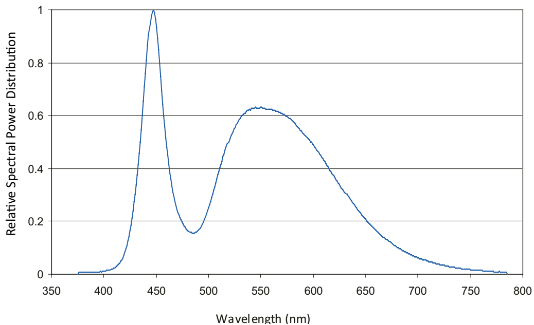
Figure 12. Color spectrum of LXML-PW3 I, LXML-PW2 I and LXML-PW1 I emitters, integrated measurement.
