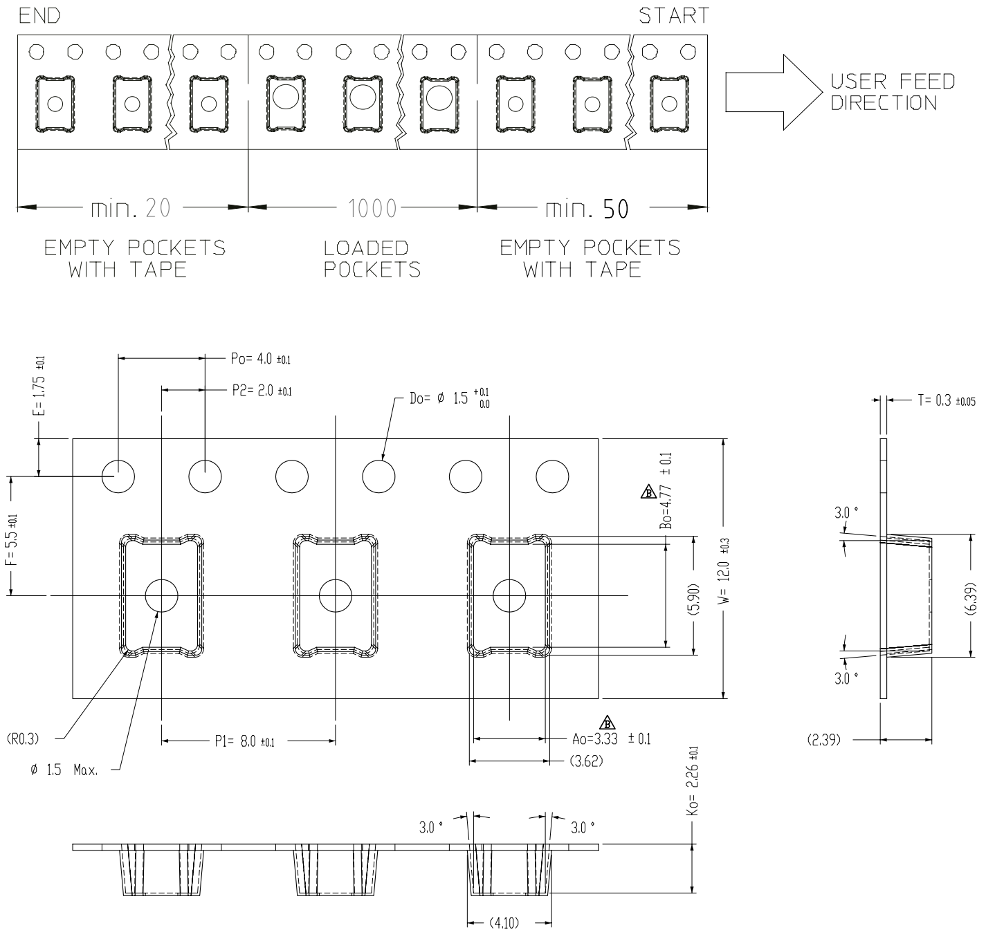
Figure 24. Emitter pocket tape packaging.
