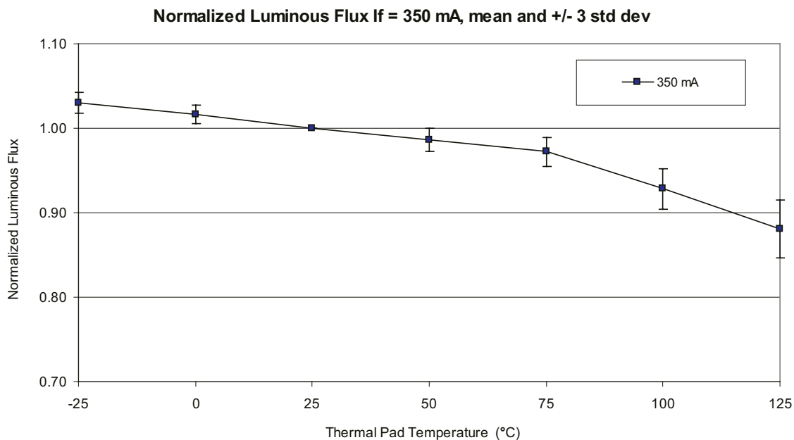
Figure 13. Relative light output vs. thermal pad temperature.
