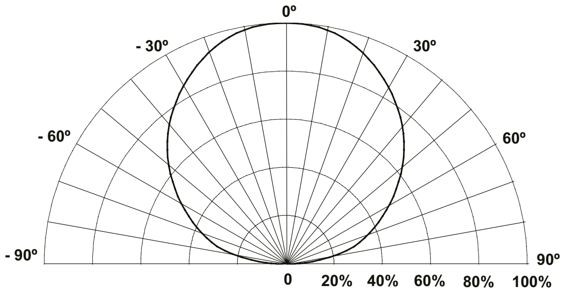
Figure 21. Typical polar radiation pattern for lambertian.
