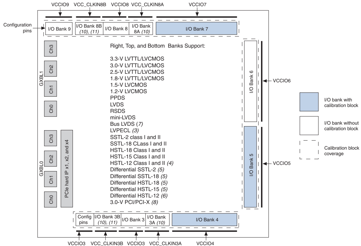
Figure 2–2. EP4CGX150DF31 Device I/O Bank Diagram (Note 1)
