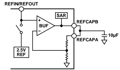
Figure 38. Reference Circuitry
