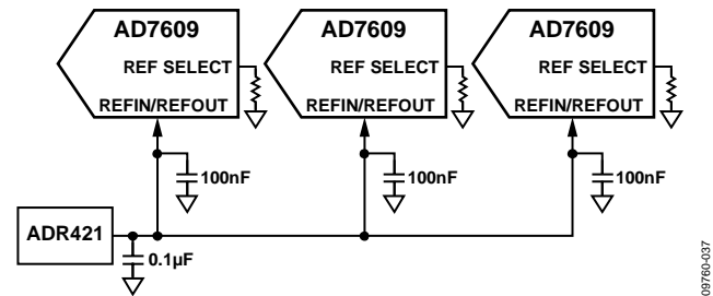
Figure 40. Internal Reference Driving Multiple AD7609 REFIN Pins
