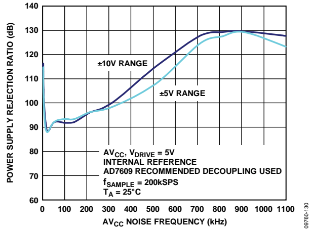
Figure 30. PSRR
