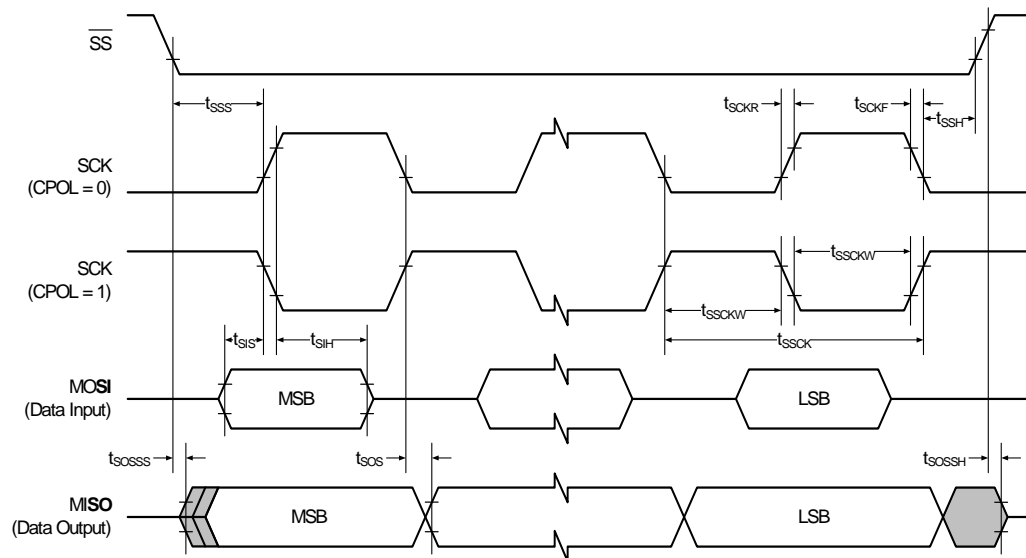
Figure 36-6. SPI timing requirements in slave mode
