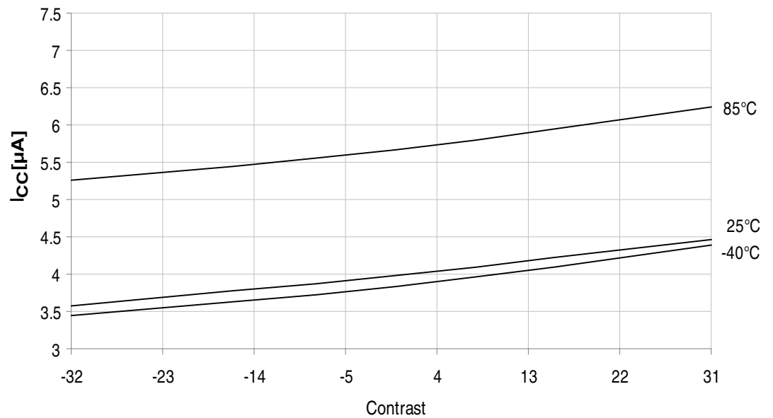
Figure 37-76. I_{CC} vs. Contrast
