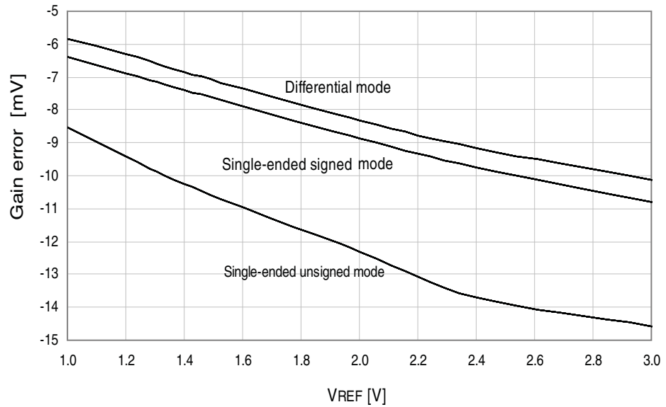
Figure 37-30. Gain error vs. V_{REF} . T = 25°C, V_{CC} = 3.6V , ADC sample rate = 300ksps.
