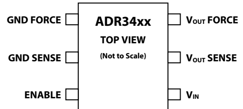
Figure 1. 6-Lead SOT23
