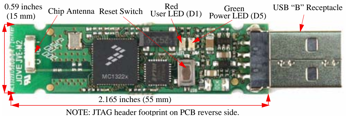
Figure 3-4. 1322x USB Dongle PCB Top View
