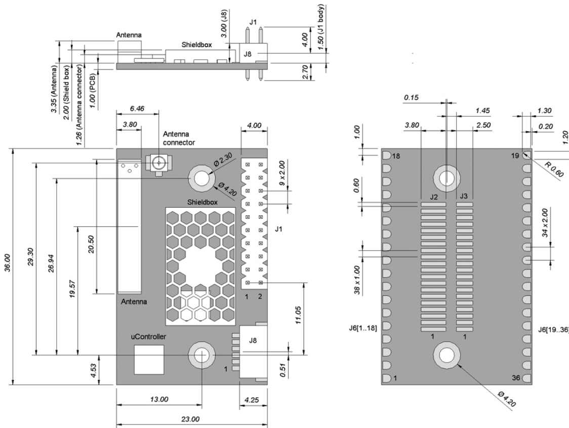
Figure 8: cB-0939 dimensions [mm].
