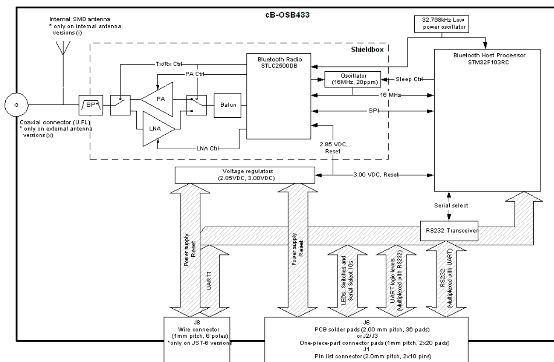
Figure 2: Block diagram of cB-0939
