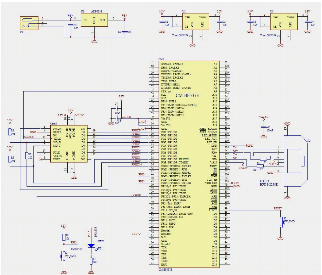
Figure 6-2: Stand-alone Ethernet based MPEG Webcam
