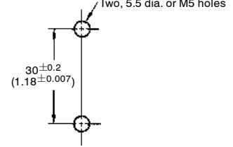
TL-N20ME/N20MY/N20MD
