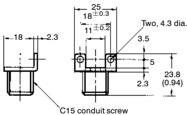
Y92E-N5C15
