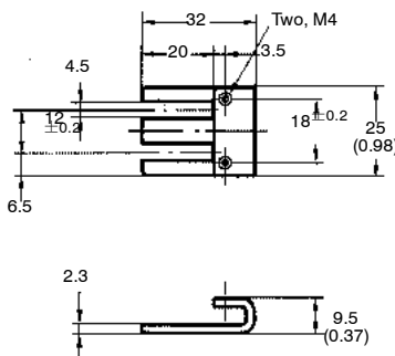
Y92E-C5
