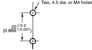
TL-N10ME/N10MY/N12MD
