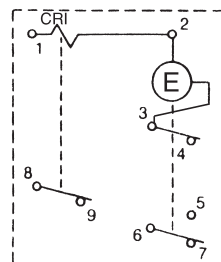
Basic Sequence of Contact Operation for BR-E "Reverse Start" Timer
