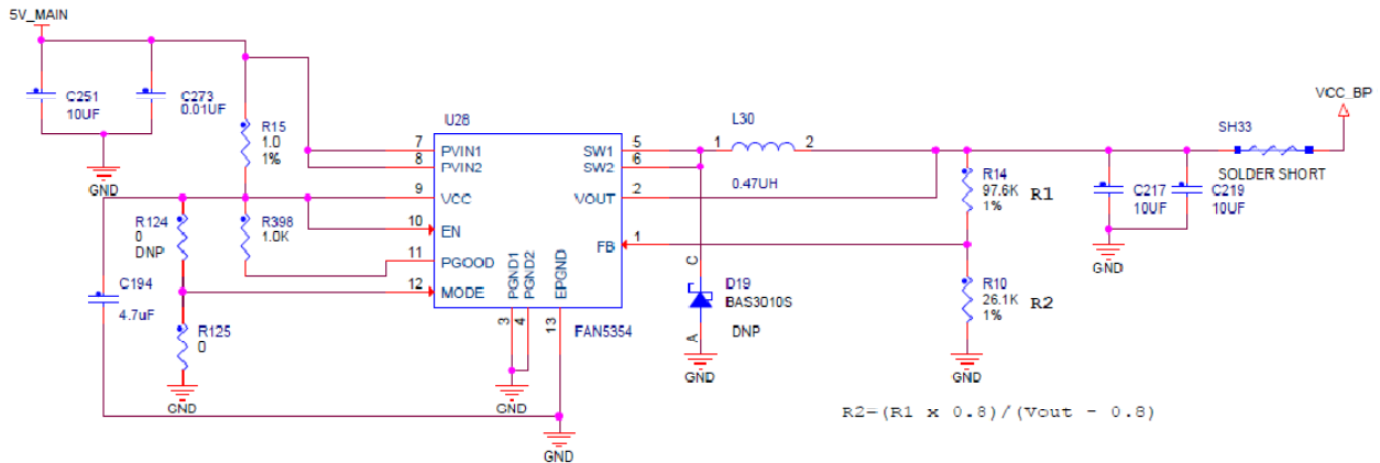
Figure 16. PMIC Main input Power Supply.
