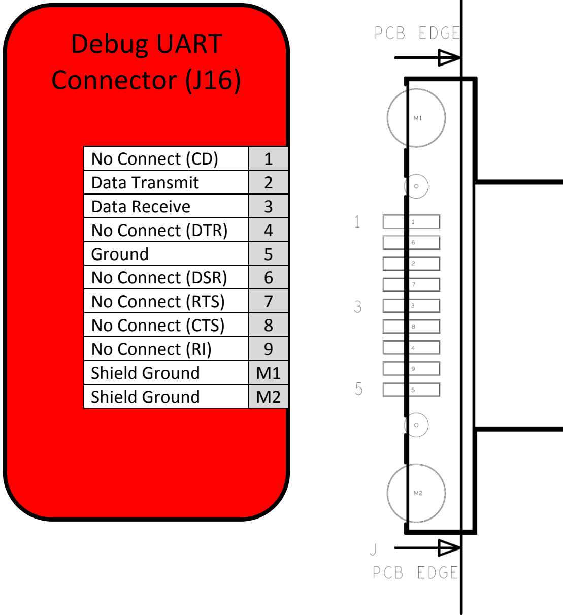
Figure 31. Debug UART Connector (J16)
