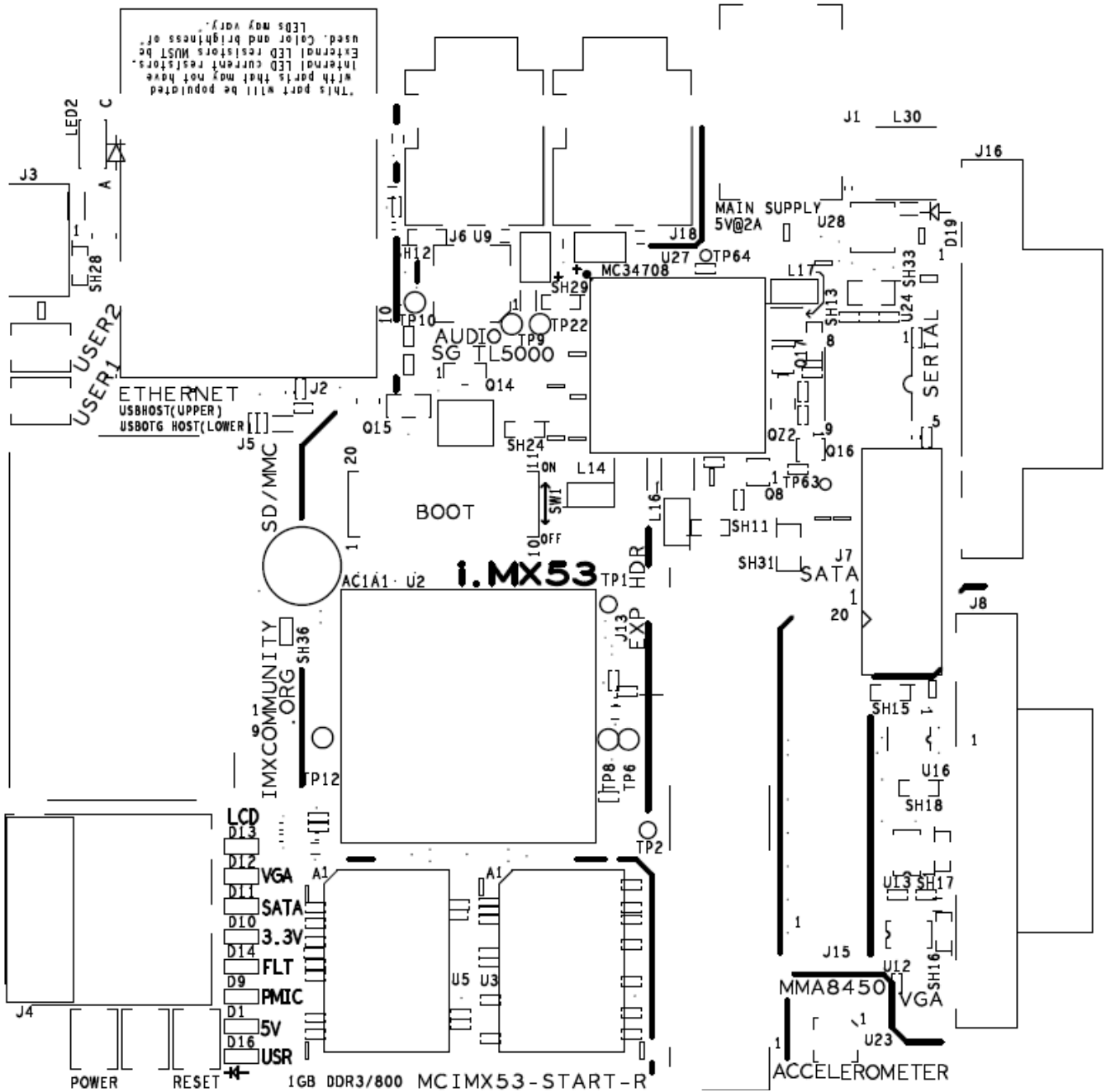
Figure 72. Silkscreen Top
