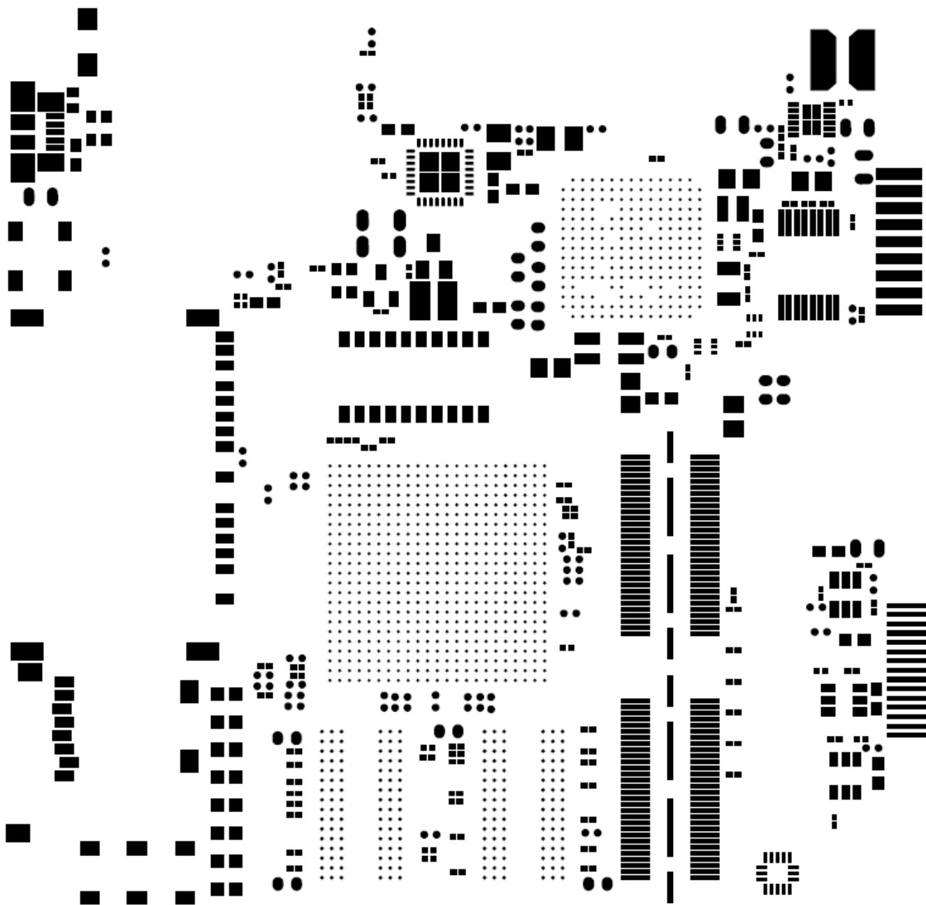
Figure 70. Pastemask Top
