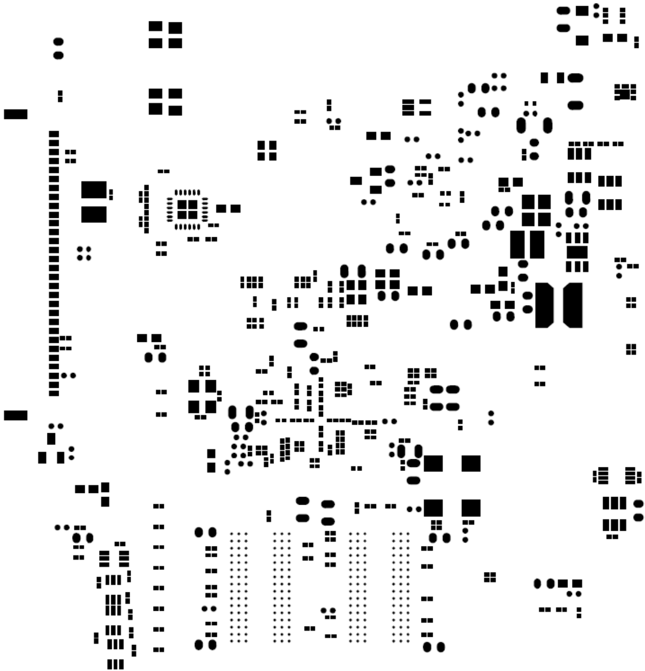
Figure 71. Pastemask Bottom
