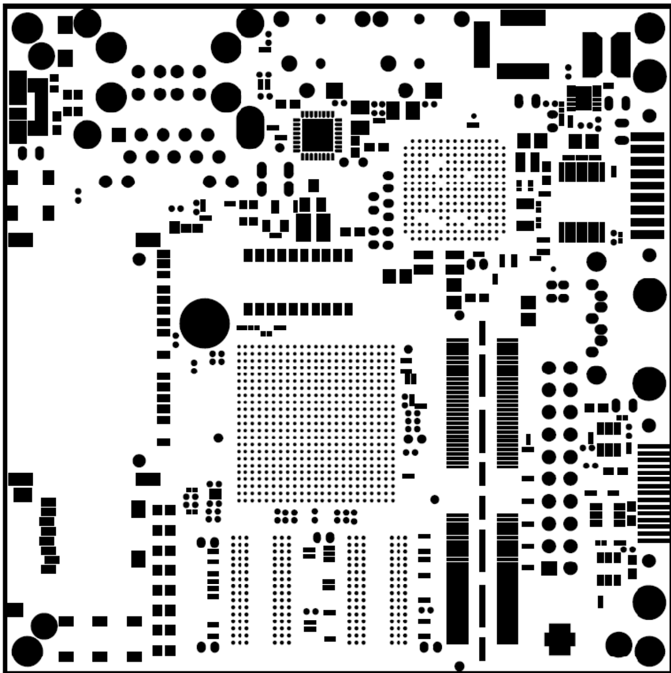
Figure 68. Soldermask Top
