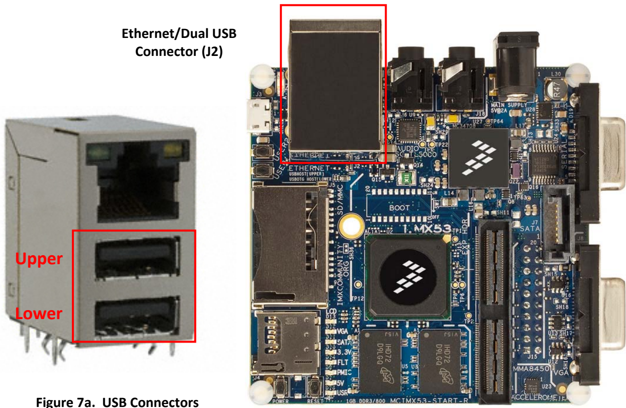
Figure 7a. USB Connectors
