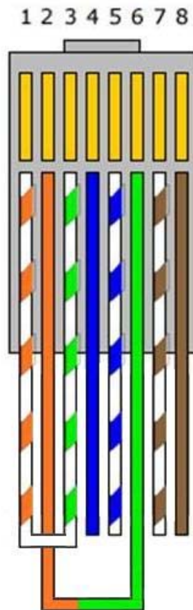
Figure 39. Ethernet Loopback Cable
