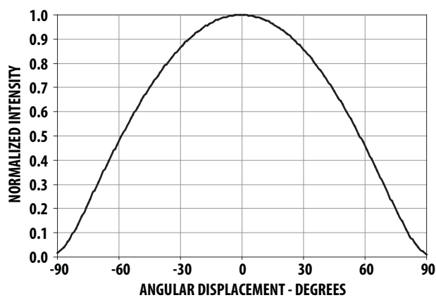
Figure 11. Radiation Pattern
