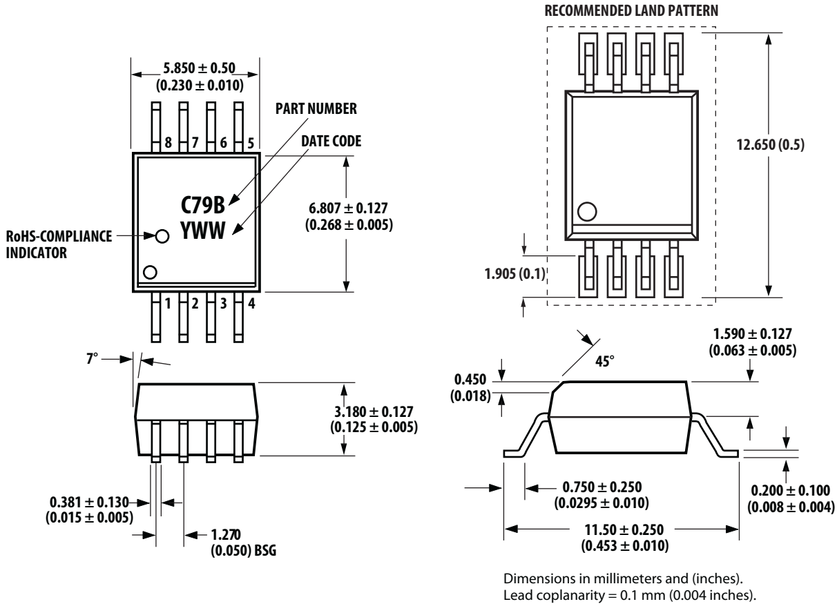
Figure 2. SS0-8 package.
