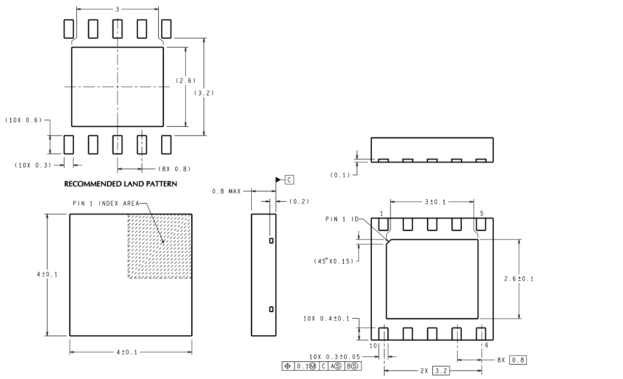
10-Lead LLP Package NS Package Number SDC10A
