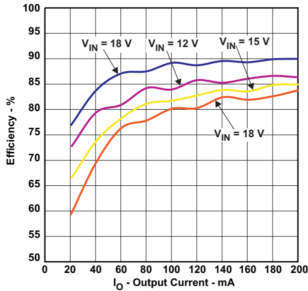
Figure 2. TPS54233EVM-373 Low Current Efficiency
