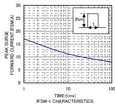
IFSM-t CHARACTERISTICS
