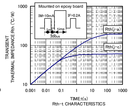
Rth-t CHARACTERISTICS
