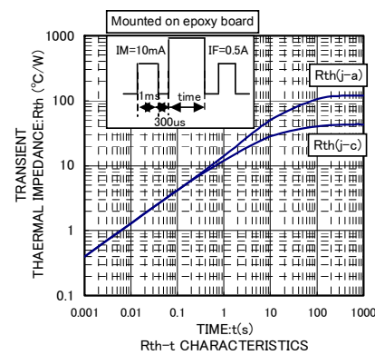
Rth-t CHARACTERISTICS
