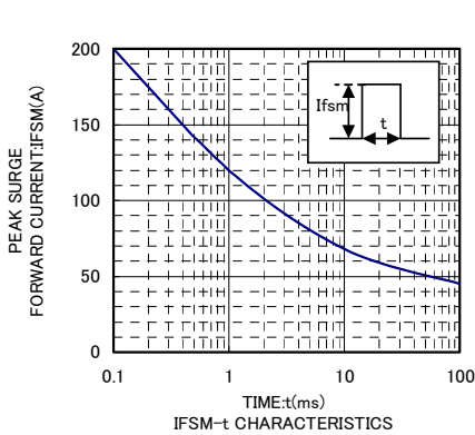
IFSM-t CHARACTERISTICS
