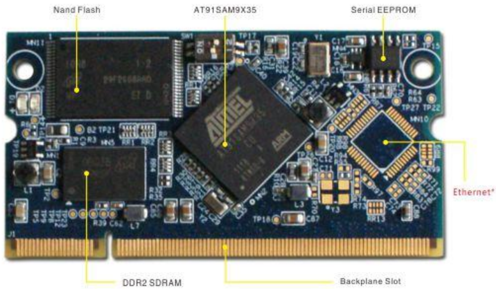
Top View
