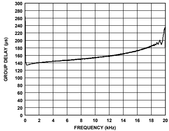
Figure 37. Group Delay vs. Frequency, f_s = 48 kHz, Signal Path = DAC_SDATA to ASRC to LOULTx
