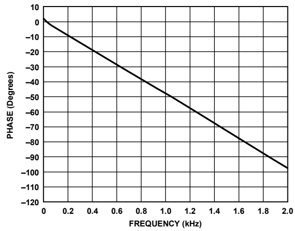
Figure 38. Phase vs. Frequency, 2 kHz Bandwidth, f_s = 48 kHz, Signal Path = DAC_SDATA to ASRC to LOULTx
