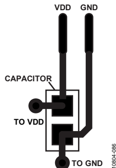
Figure 94. Recommended Power Supply Bypass Capacitor Layout
