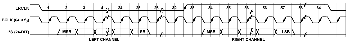
Figure 86. I 2 S Mode—16 Bits to 24 Bits per Channel
