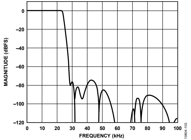
Figure 62. Total Decimation Response, f_s = 192 kHz
