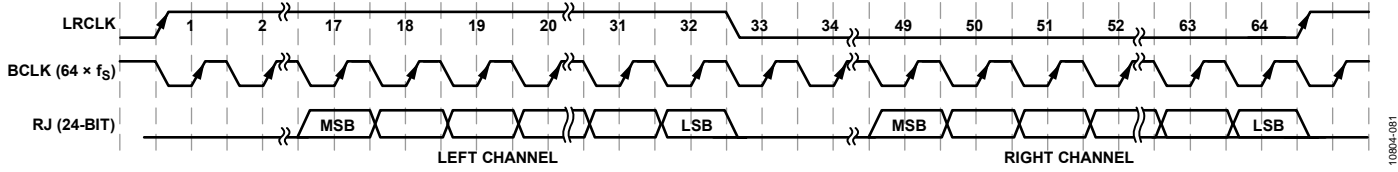
Figure 89. Right Justified Mode—16 Bits per Channel
