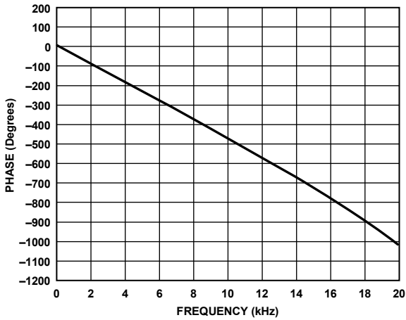
Figure 23. Phase vs. Frequency, 20 kHz Bandwidth, f_s = 48 kHz, Signal Path = AIN0 to ASRC to ADC_SDATA0
