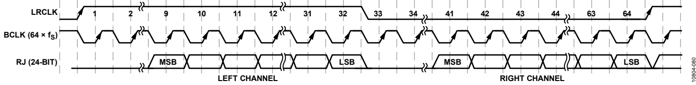
Figure 88. Right Justified Mode—24 Bits per Channel
