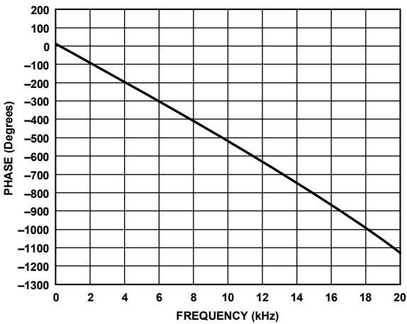
Figure 35. Phase vs. Frequency, 20 kHz Bandwidth, f_s = 48 kHz, Signal Path = DAC_SDATA to ASRC to LOULTx
