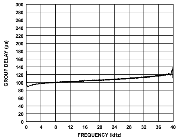
Figure 39. Group Delay vs. Frequency, f_s = 96 kHz, Signal Path = DAC_SDATA to ASRC to LOULTx
