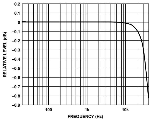
Figure 36. Relative Level vs. Frequency, f_s = 96 kHz, Signal Path = DAC_SDATA to ASRC to LOULTx
