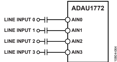
Figure 71. Single-Ended Line Inputs
