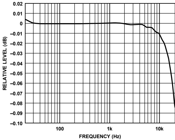
Figure 34. Relative Level vs. Frequency, f_s = 48 kHz, Signal Path = DAC_SDATA to ASRC to LOULTx
