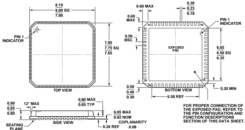
Figure 78. 56-Lead Lead Frame Chip Scale Package [LFCSP_VQ] 8 mm × 8 mm Body, Very Thin Quad (CP-56-3) Dimensions shown in millimeters
