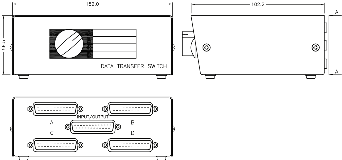
View: A-A
