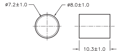
INSULATION TUBE
