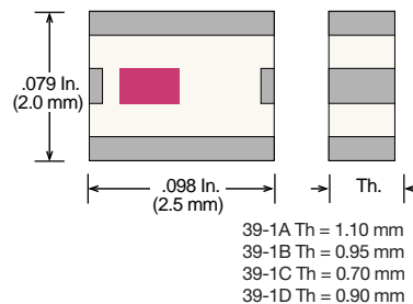
Case 39-1 (2520)
