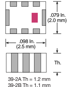
Case 39-2 (2520)
