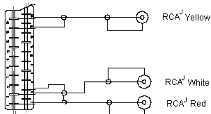
Wiring Diagram (8226 Out)
