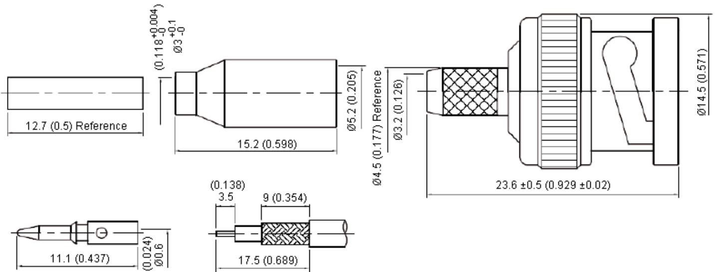
Stripping Dimension
