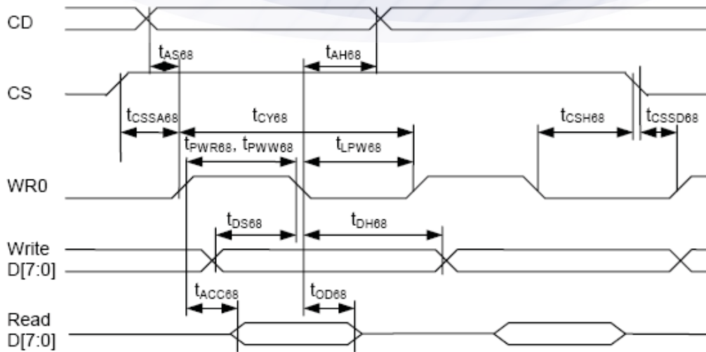
Parallel Bus Timing Characteristics (for 6800 MCU)
