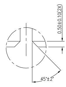
DETAIL B SCALE 5:1
