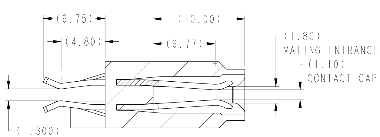
SECTION C-C
