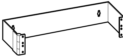
2U Shallow Wall-Mount Rack Dimensions: 89mm x 495mm x 102mm (3.5"H x 19.5"W x 4"D) Shipping Weight: 1.4kg (3 lb.)
