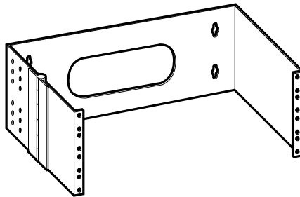
4U Deep Wall-Mount Rack Dimensions: 178mm x 489mm x 203mm (7"H x 19.25"W x 8"D) Shipping Weight: 2.3kg (5 lb.)
