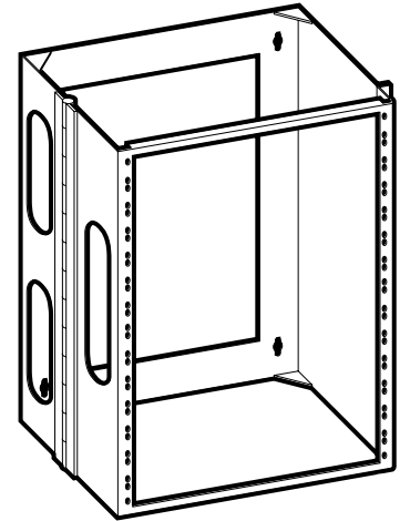
14U Deep Wall-Mount Rack Dimensions: 648mm x 489mm x 203mm (25.5"H x 19.25"W x 8"D) Shipping Weight: 12.7kg (28 lb.)
