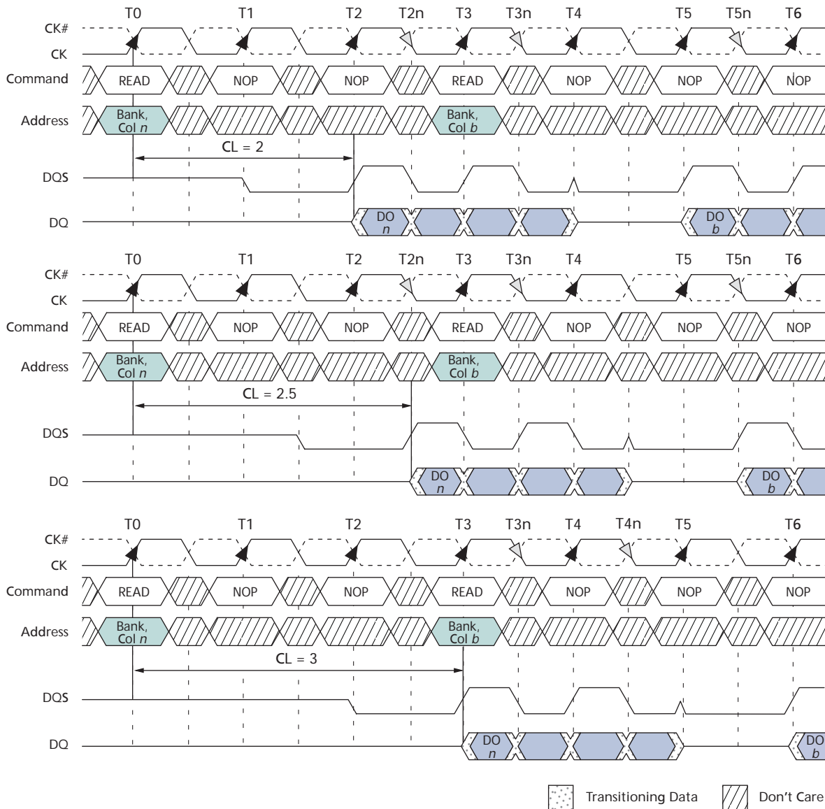
Figure 20: Nonconsecutive READ Bursts
