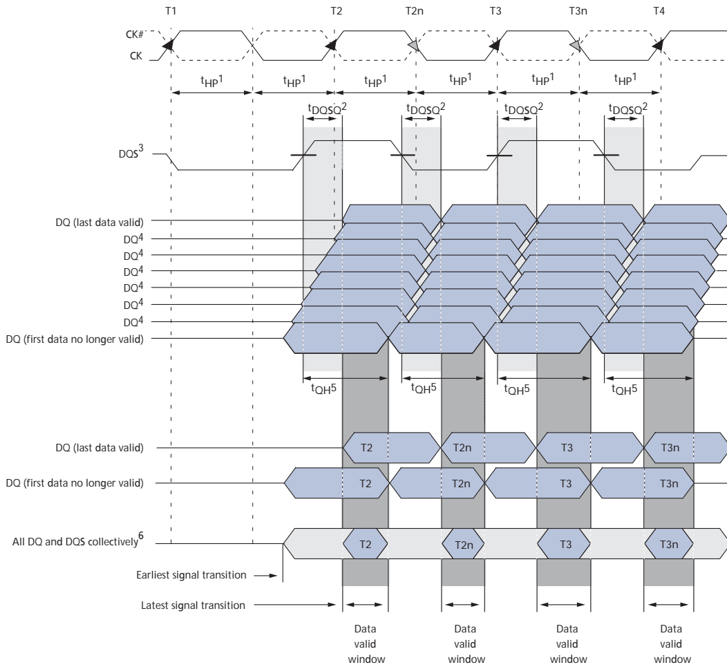
Figure 26: x4, x8 Data Output Timing – t_{DQSQ} , t_{QH} , and Data Valid Window
