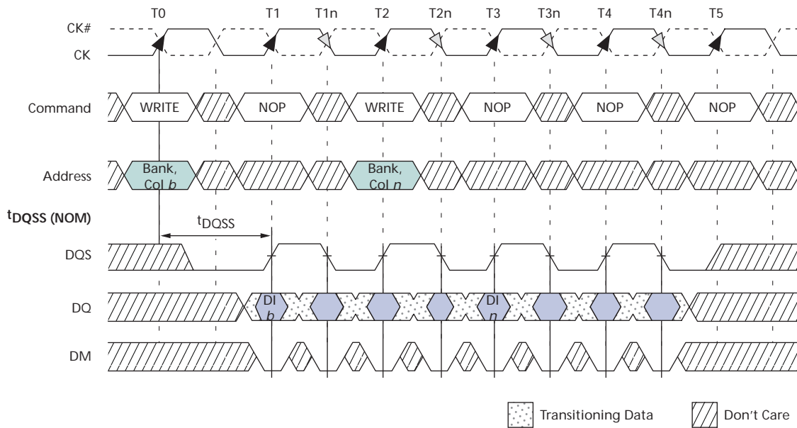
Figure 30: Consecutive WRITE-to-WRITE
