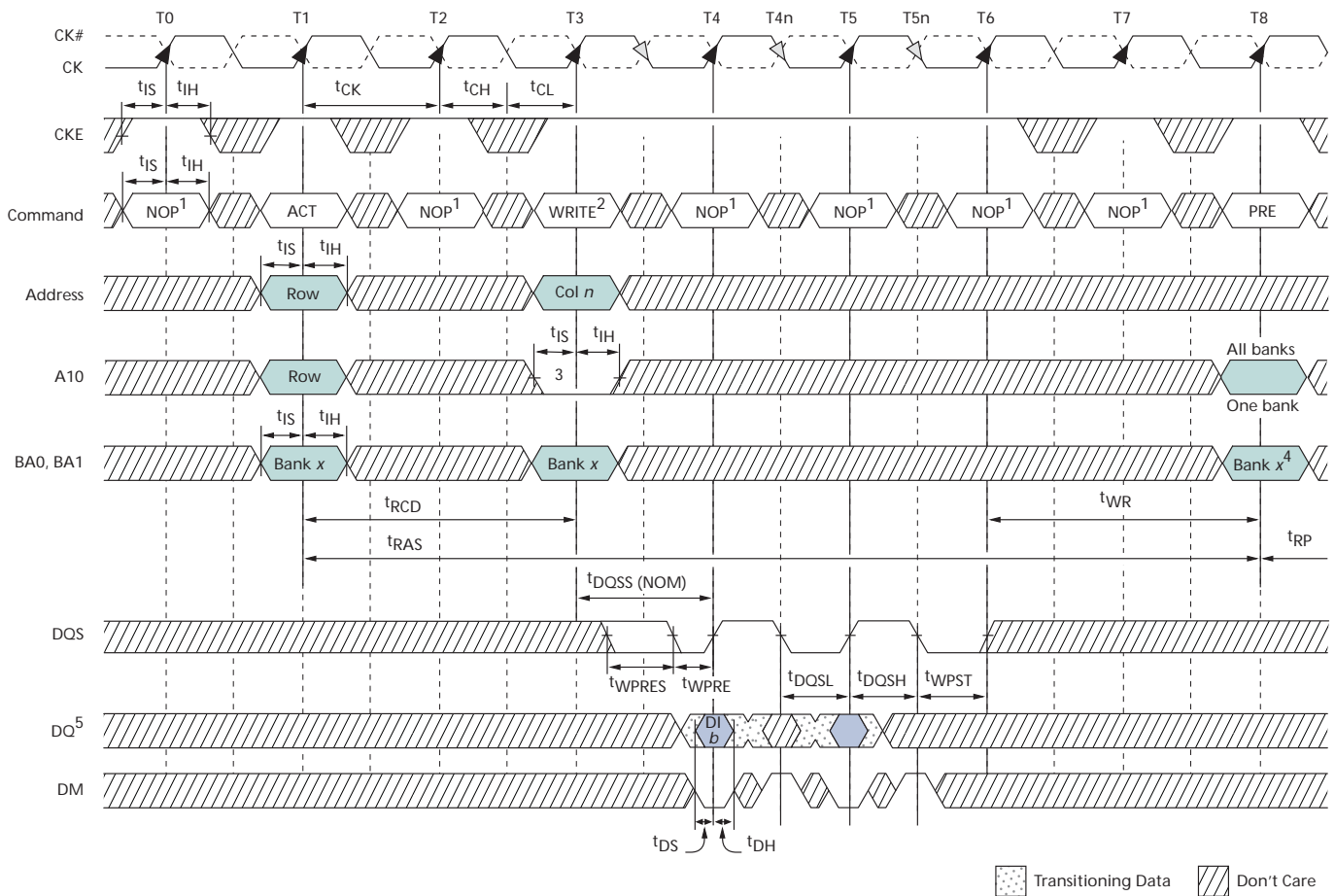
Figure 40: WRITE - DM Operation
