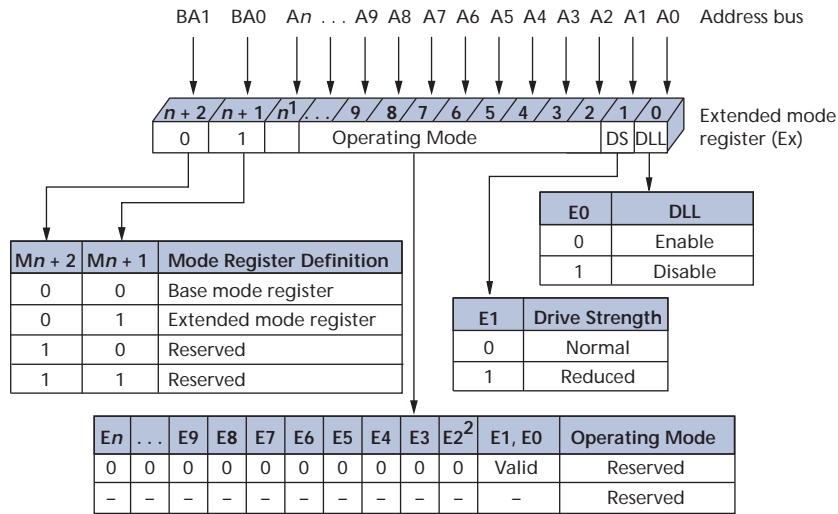
Figure 16: Extended Mode Register Definition
