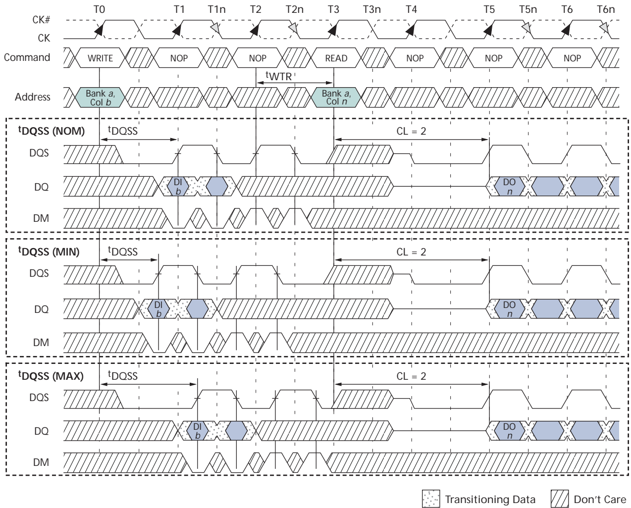
Figure 34: WRITE-to-READ - Interrupting
