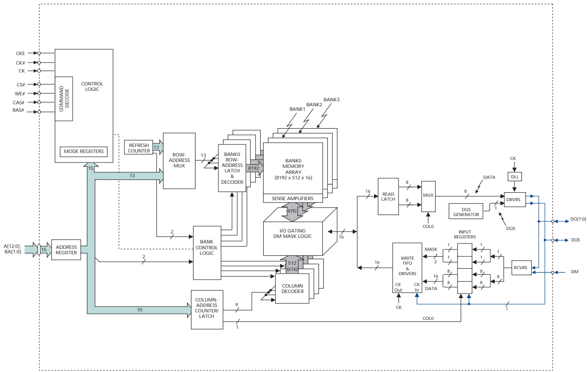
Figure 3: 16 Meg x 16 Functional Block Diagram
