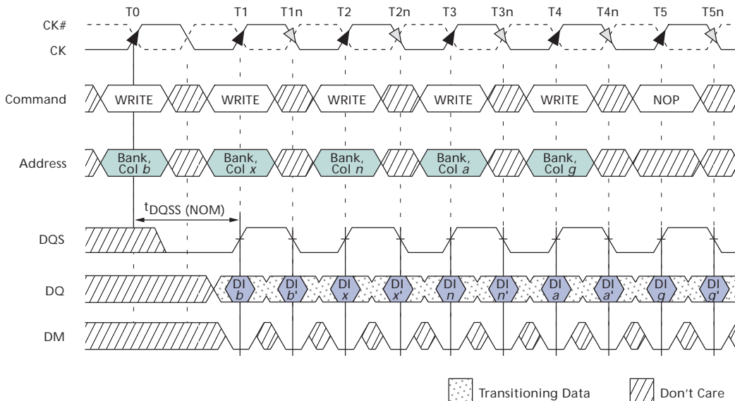
Figure 32: Random WRITE Cycles
