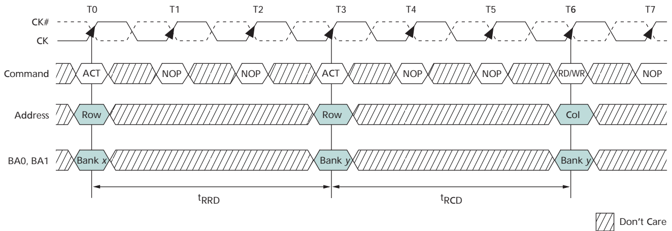
Figure 17: Example: Meeting t_{RCD} ( t_{RRD} ) MIN When 2 < t_{RCD} ( t_{RRD} ) MIN/ t_{CK} \leq 3
