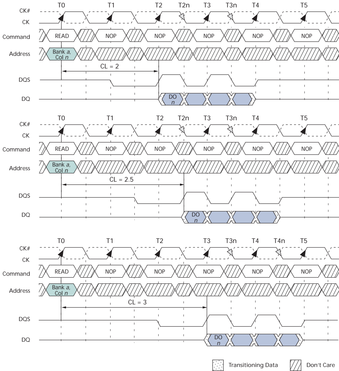
Figure 18: READ Burst
