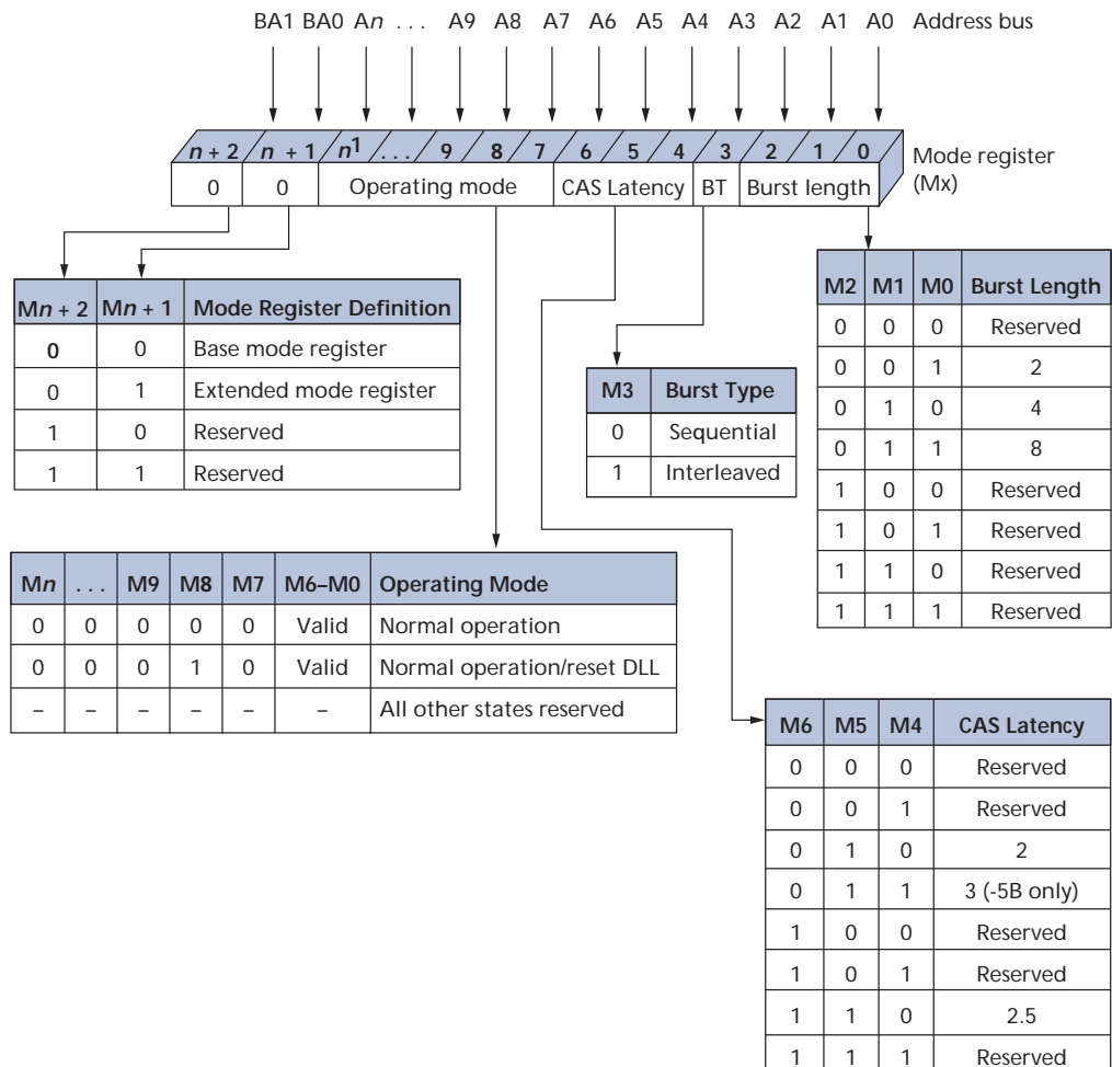
Figure 14: Mode Register Definition
