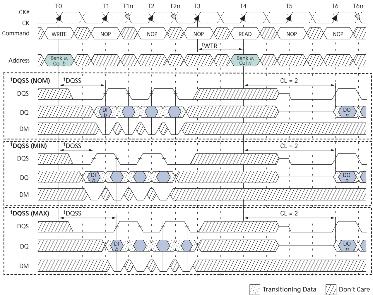
Figure 33: WRITE-to-READ – Uninterrupting
