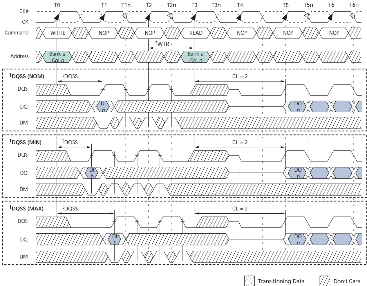
Figure 35: WRITE-to-READ – Odd Number of Data, Interrupting
