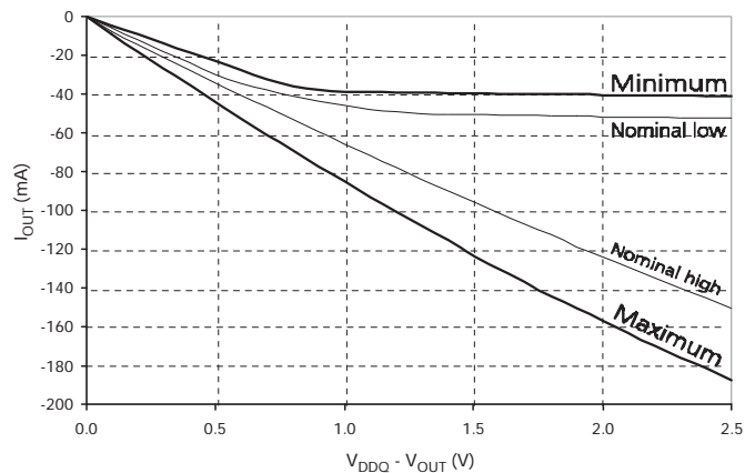
Figure 5: Full Drive Pull-Up Characteristics
