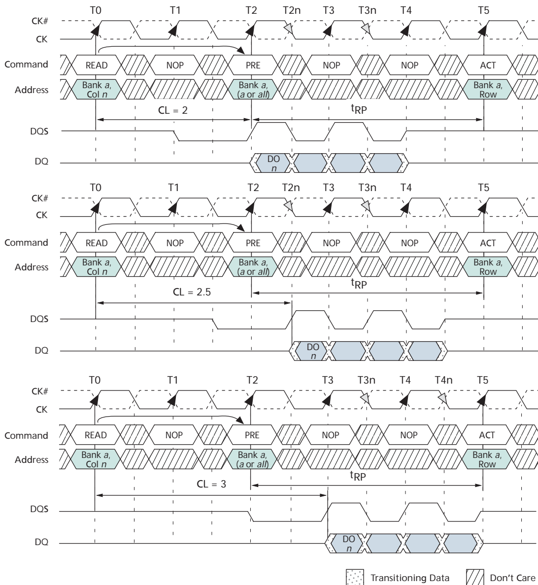
Figure 24: READ-to-PRECHARGE
