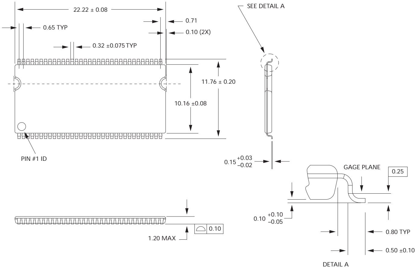
Figure 6: 66-Pin Plastic TSOP (400 mil)
