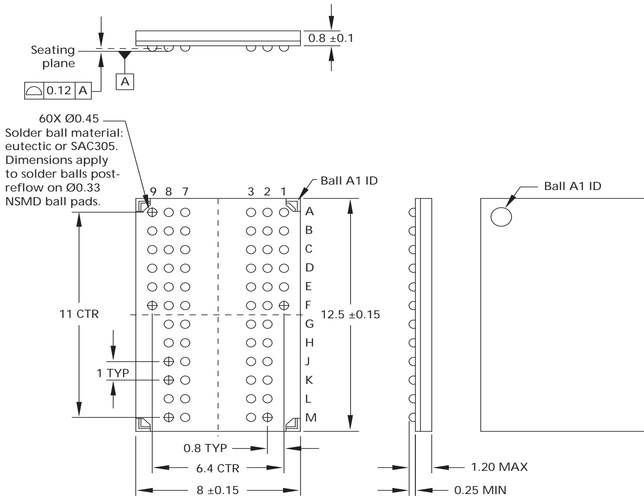
Figure 7: 60-Ball FBGA (8mm x 12.5mm)
