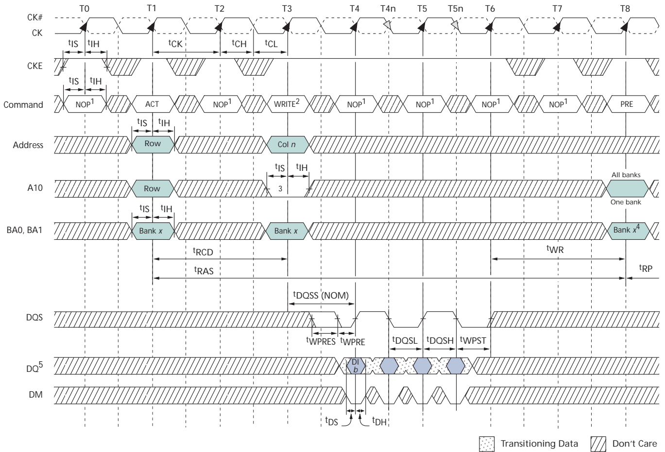
Figure 39: Bank WRITE – Without Auto Precharge
