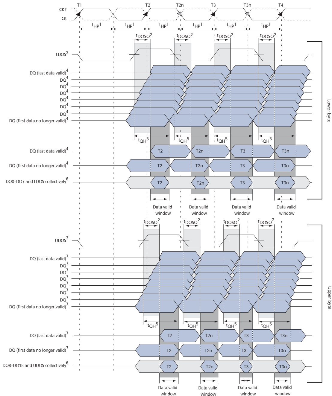
Figure 27: x16 Data Output Timing – t_{DQSQ} , t_{QH} , and Data Valid Window
