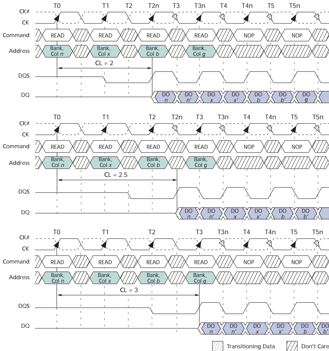
Figure 21: Random READ Accesses
