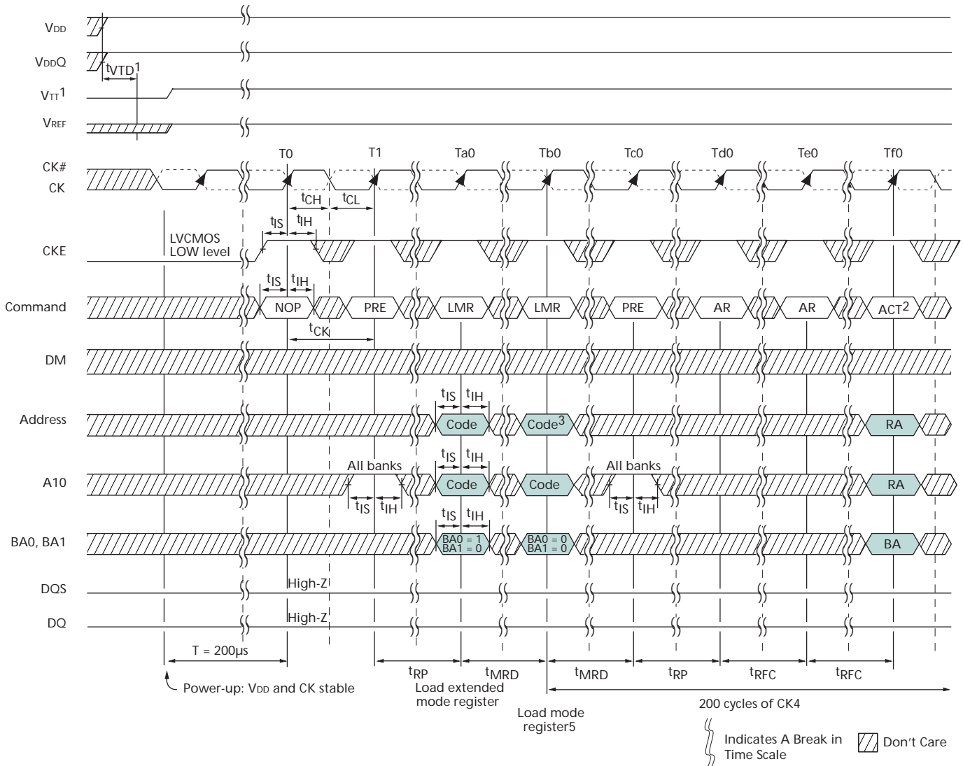
Figure 13: INITIALIZATION Timing Diagram
