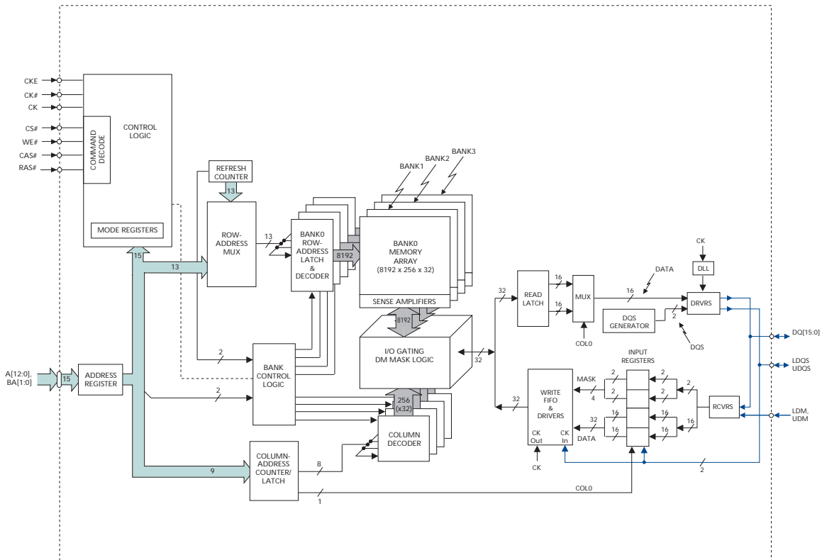
Figure 3: 16 Meg x 16 Functional Block Diagram
