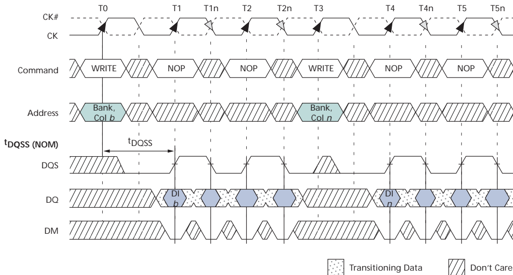
Figure 31: Nonconsecutive WRITE-to-WRITE
