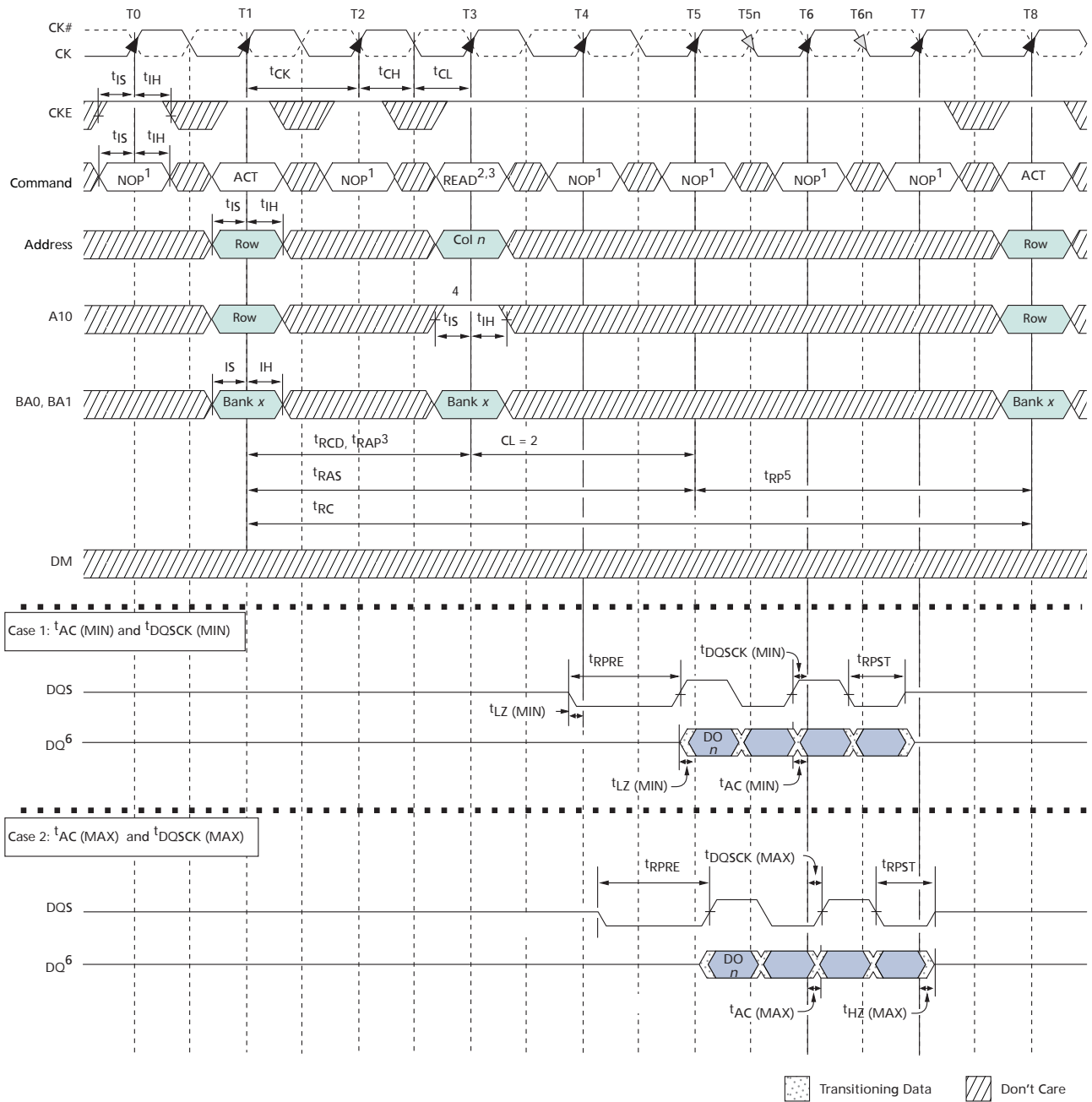
Figure 42: Bank READ - with Auto Precharge
