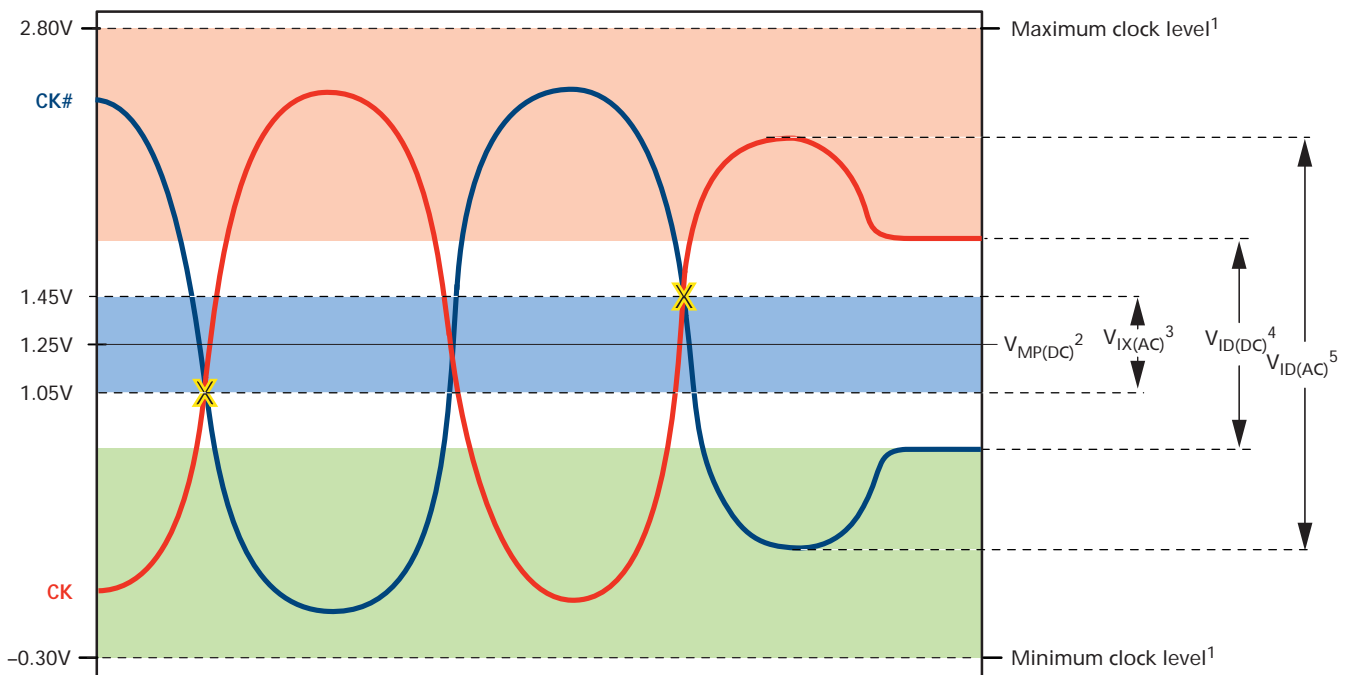
Figure 2: SSTL_2 Clock Input
