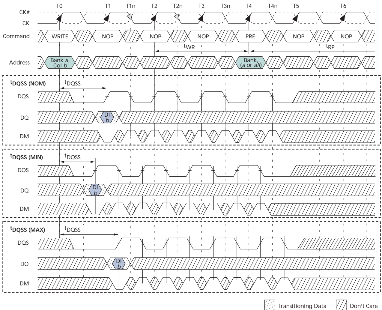
Figure 38: WRITE-to-PRECHARGE - Odd Number of Data, Interrupting
