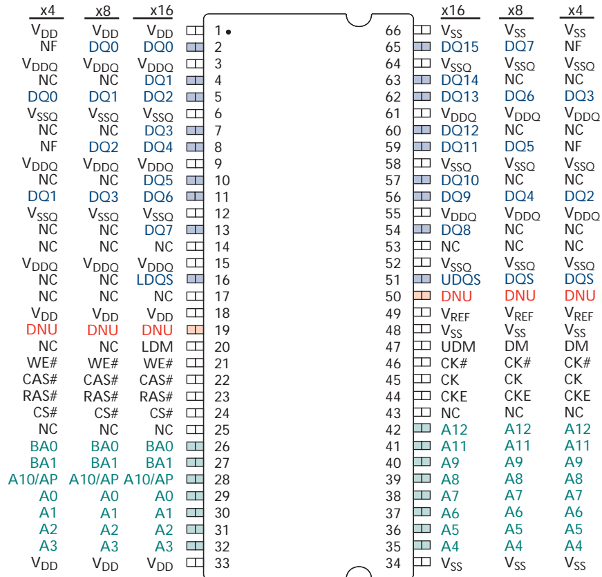
Figure 4: 66-Pin TSOP Pin Assignments (Top View)
