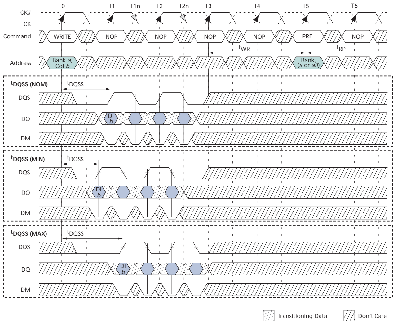
Figure 36: WRITE-to-PRECHARGE - Uninterrupting
