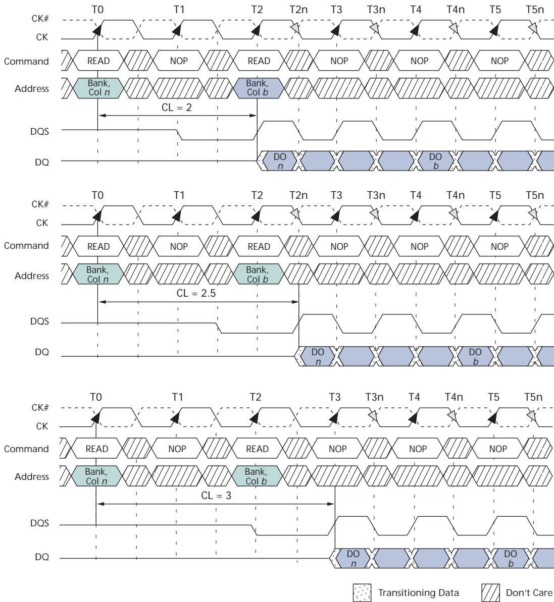
Figure 19: Consecutive READ Bursts
