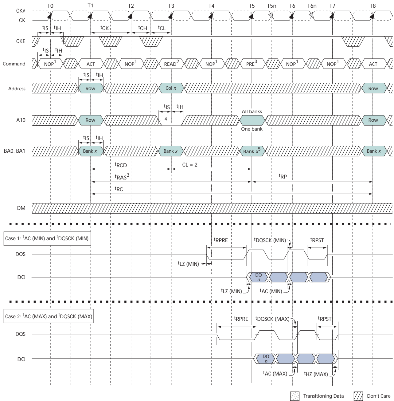
Figure 25: Bank READ – Without Auto Precharge
