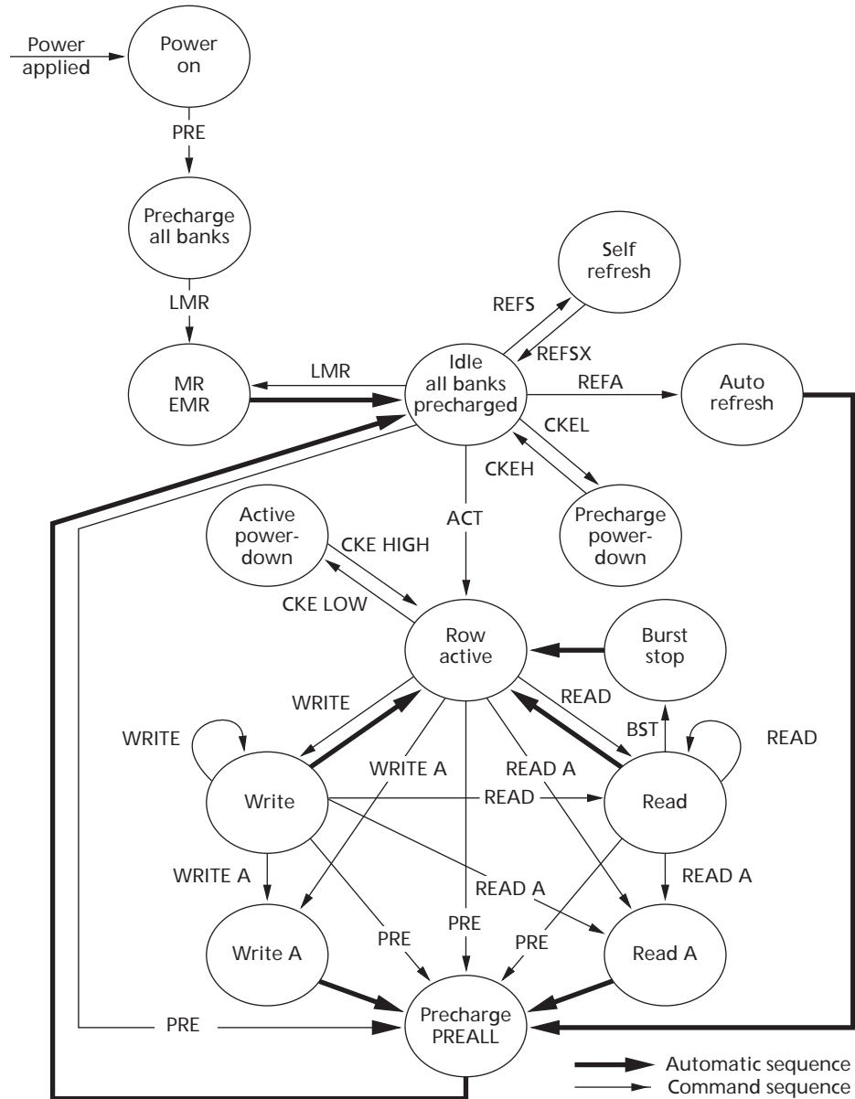
Figure 1: Simplified State Diagram
