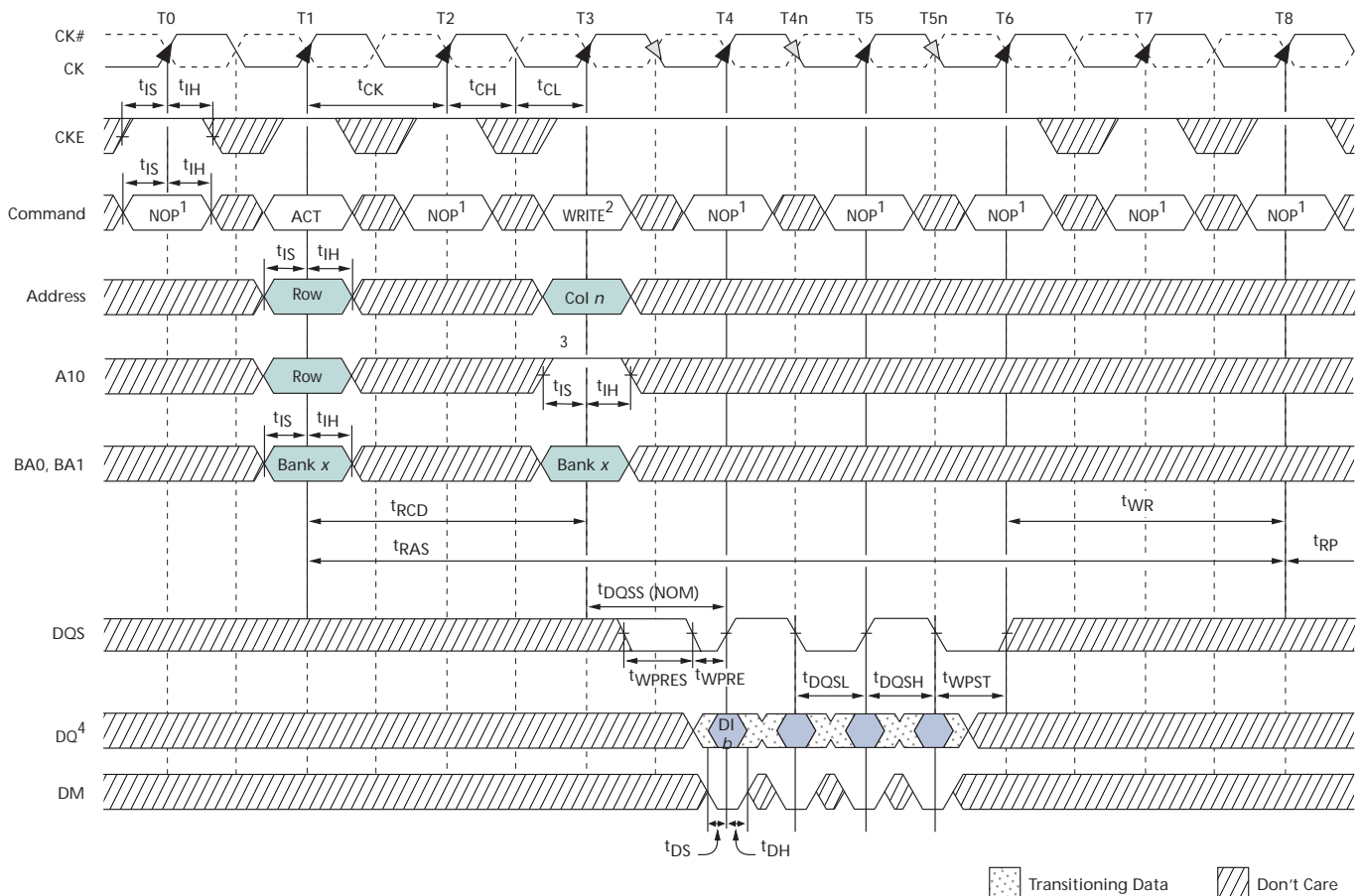
Figure 43: Bank WRITE – with Auto Precharge
