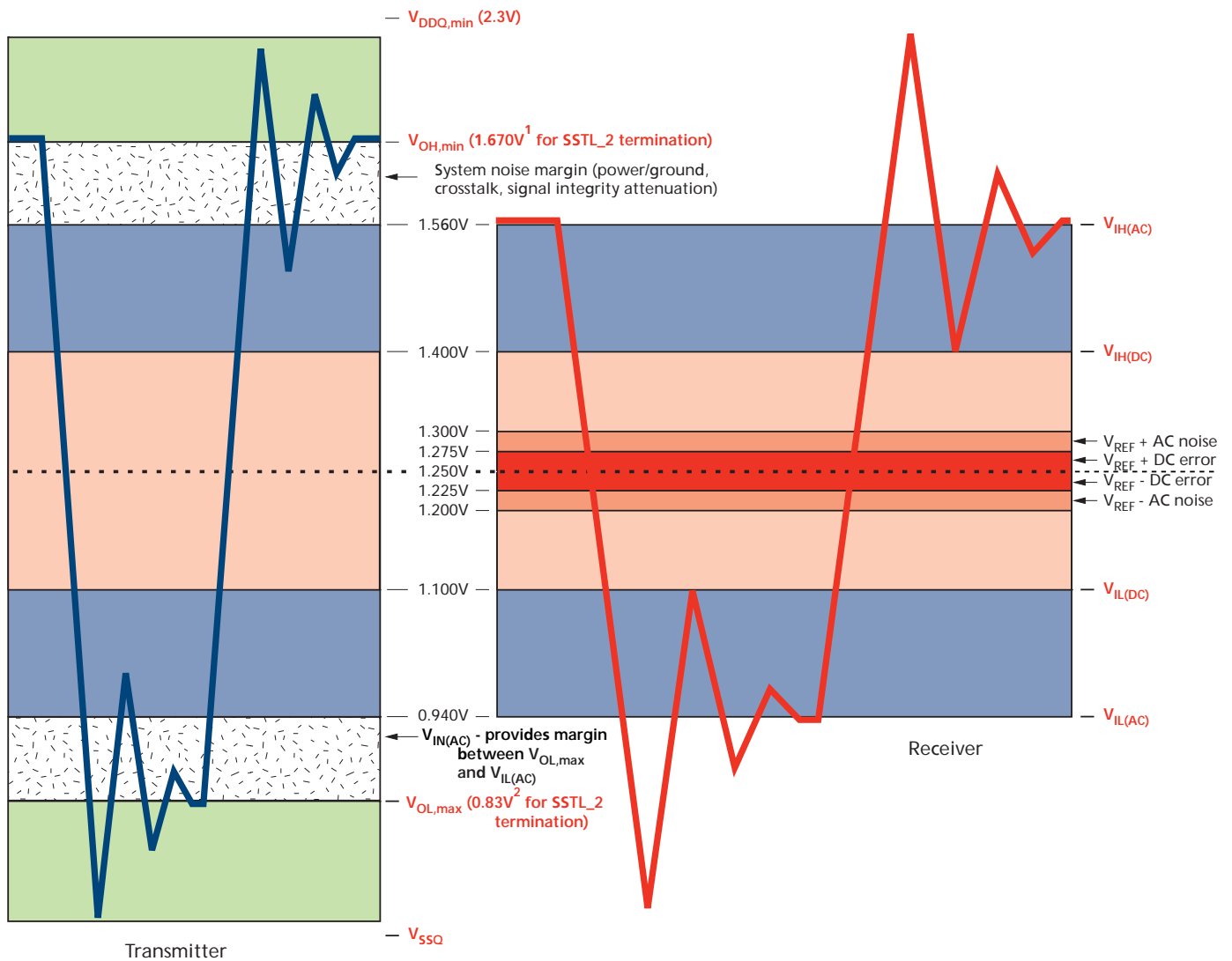
Figure 1: Input Voltage Waveform
