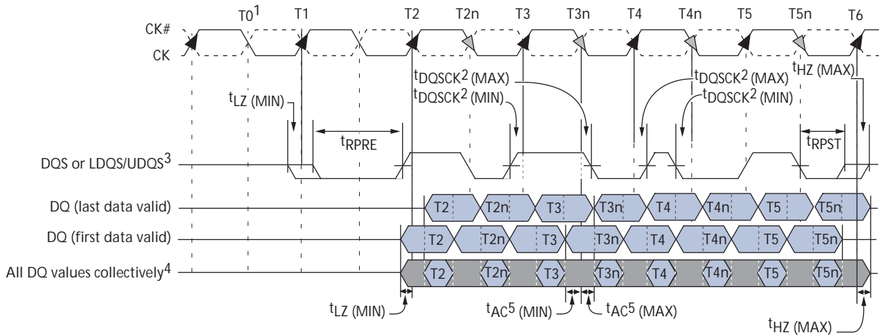
Figure 28: Data Output Timing – t_{AC} and t_{DQSK}
