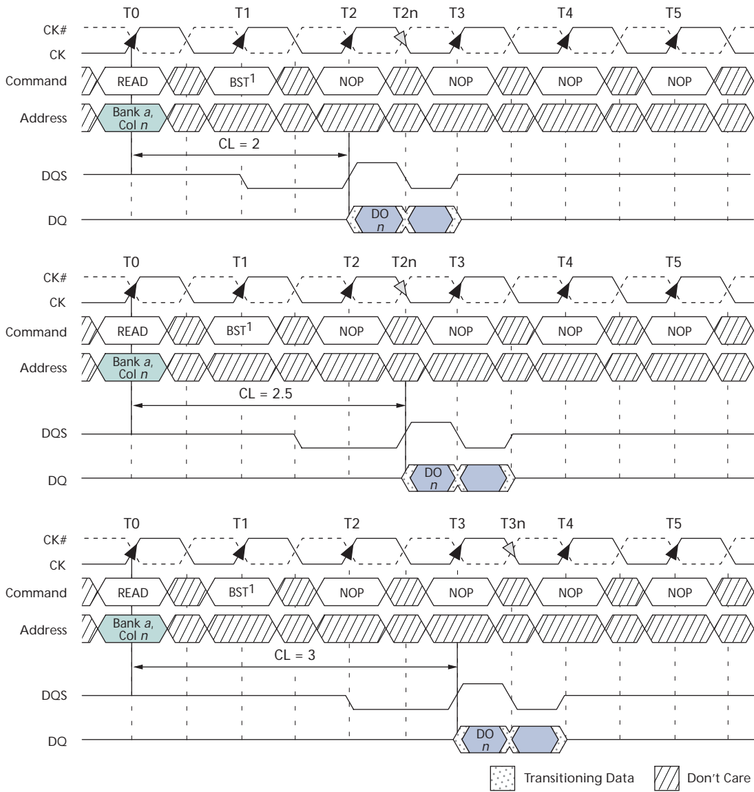
Figure 22: Terminating a READ Burst
