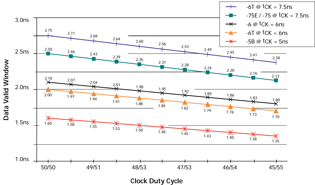
Figure 3: Derating Data Valid Window ( t_{QH} - t_{DQSQ} )
