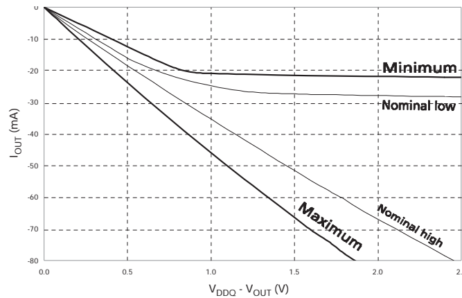
Figure 7: Reduced Drive Pull-Up Characteristics
