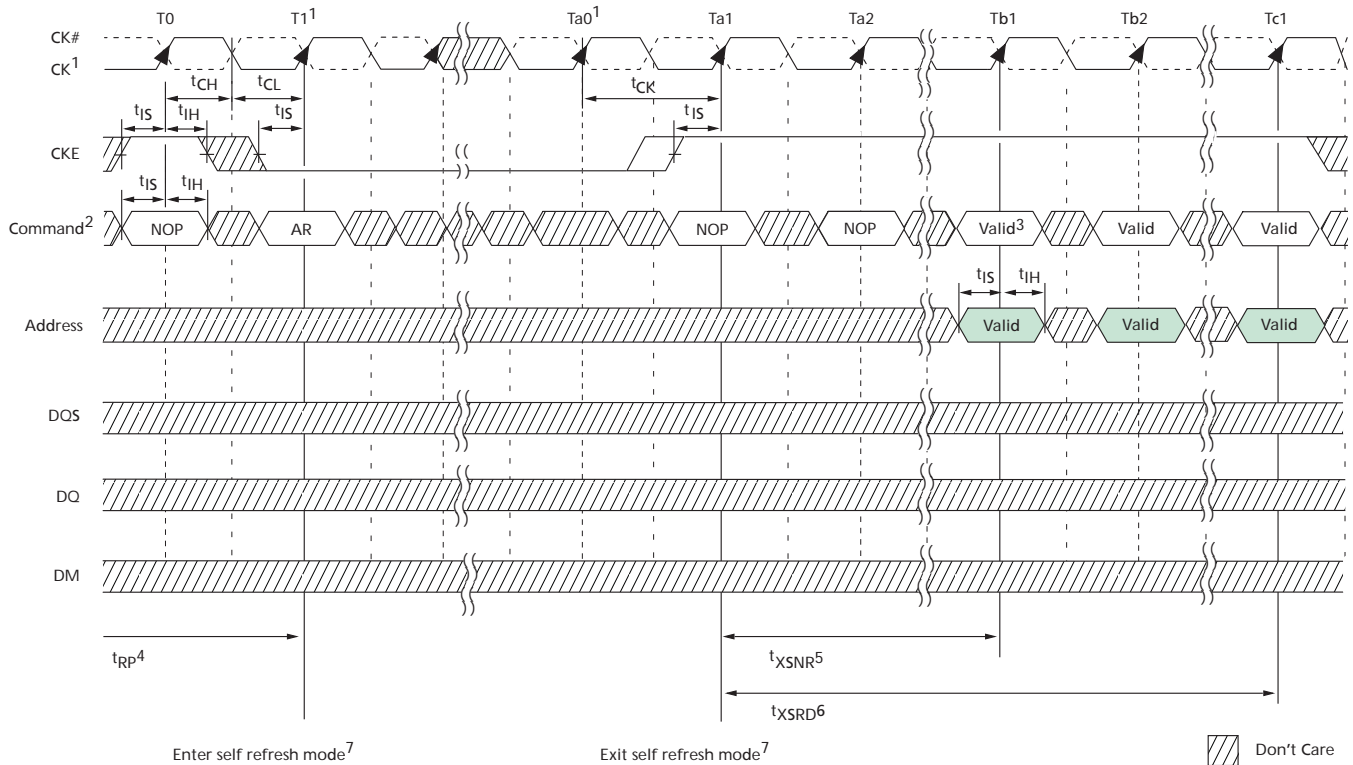
Figure 45: Self Refresh Mode
