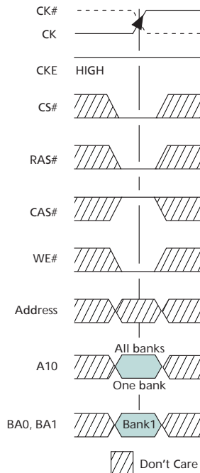
Figure 11: PRECHARGE Command
