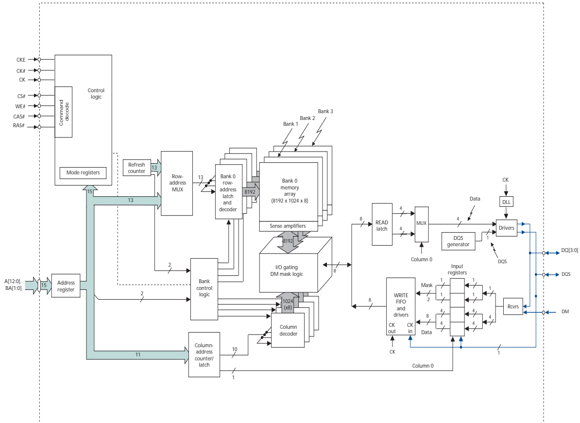
Figure 1: 64 Meg x 4 Functional Block Diagram
