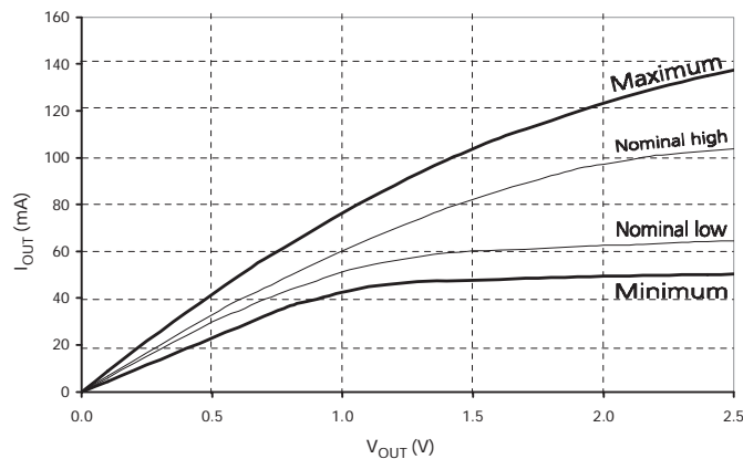
Figure 5: Full Drive Pull-Up Characteristics
