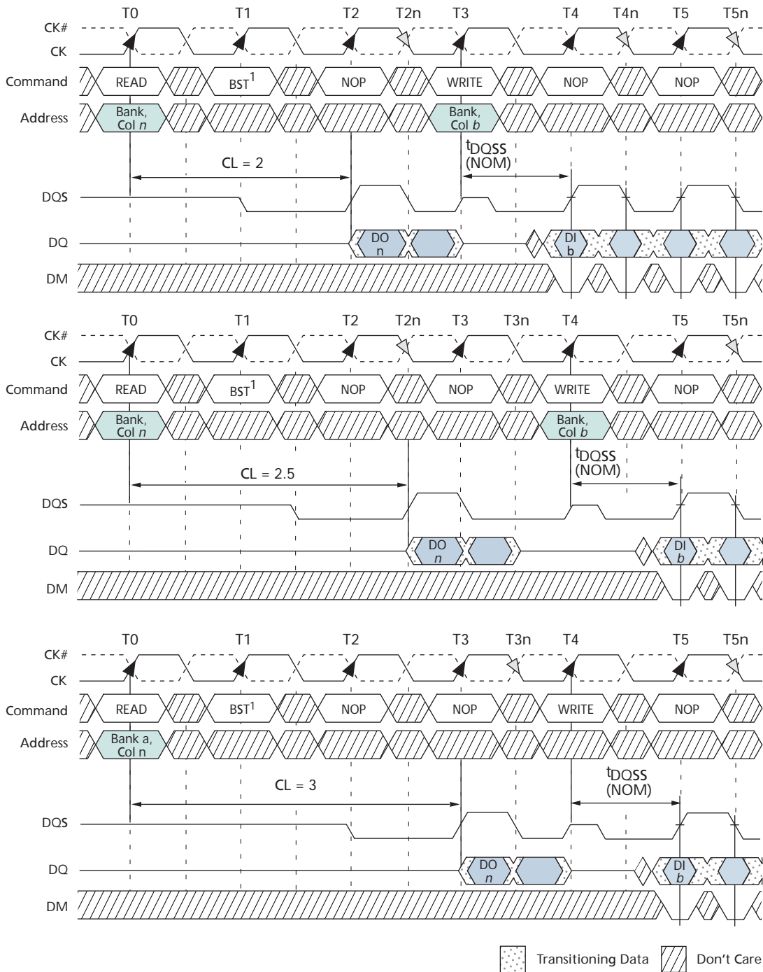
Figure 23: READ-to-WRITE
