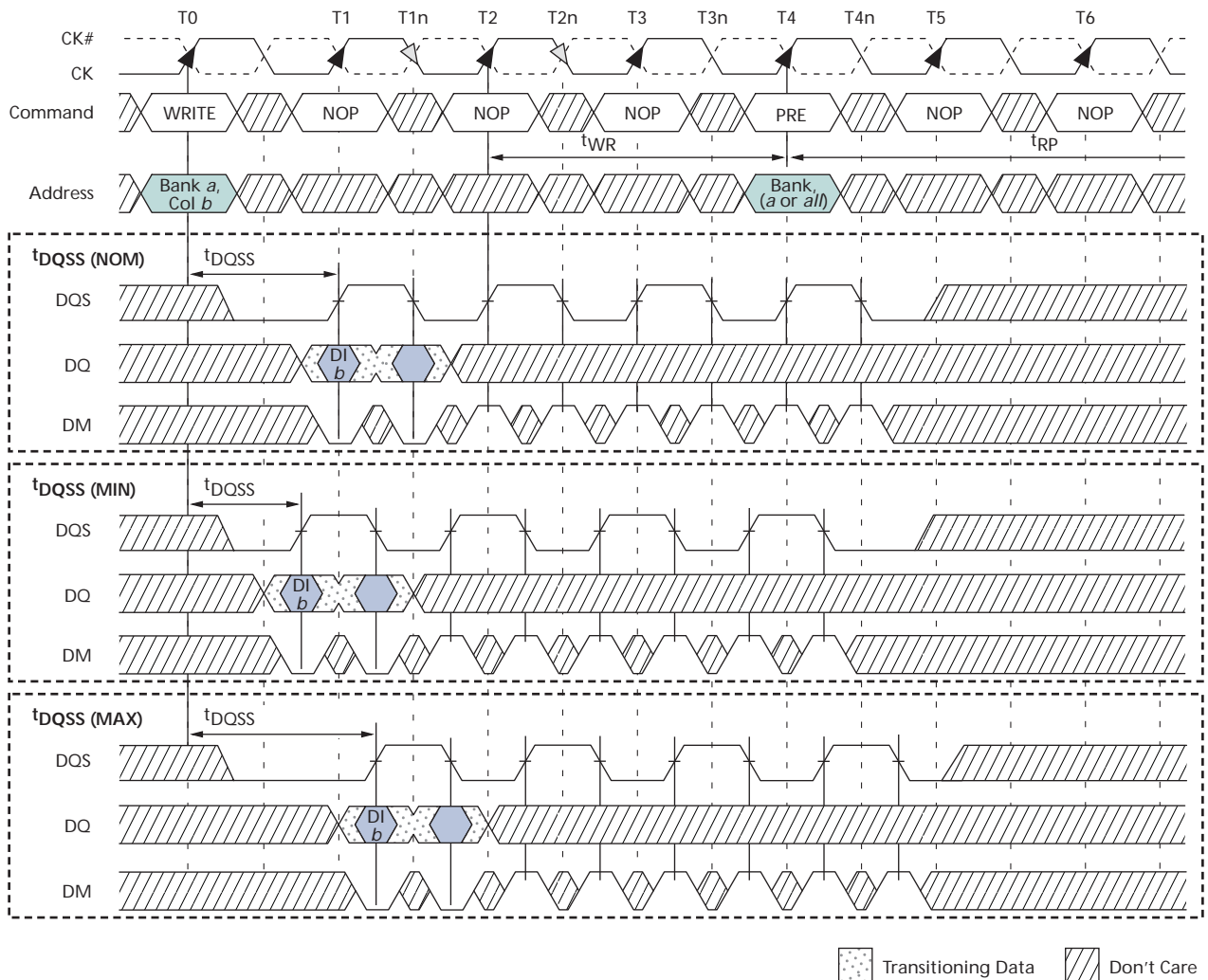
Figure 37: WRITE-to-PRECHARGE - Interrupting
