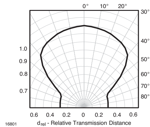
Figure 12. Directivity
