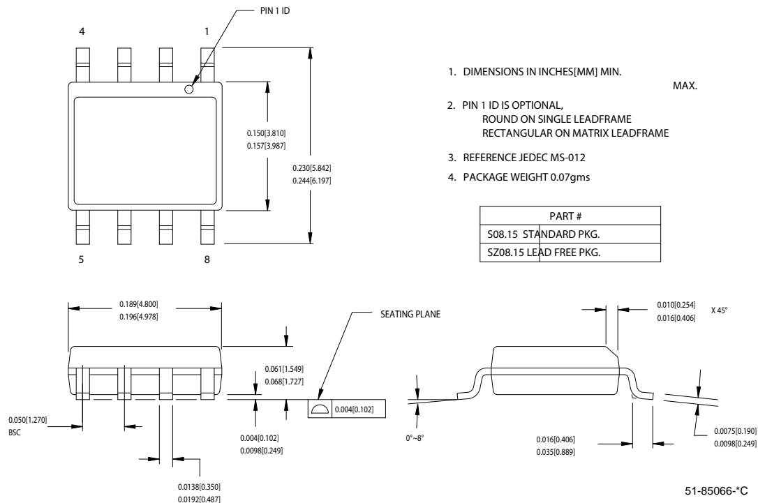
Figure 5. 8-Pin (150-Mil) SOIC S8 (51-85066)
