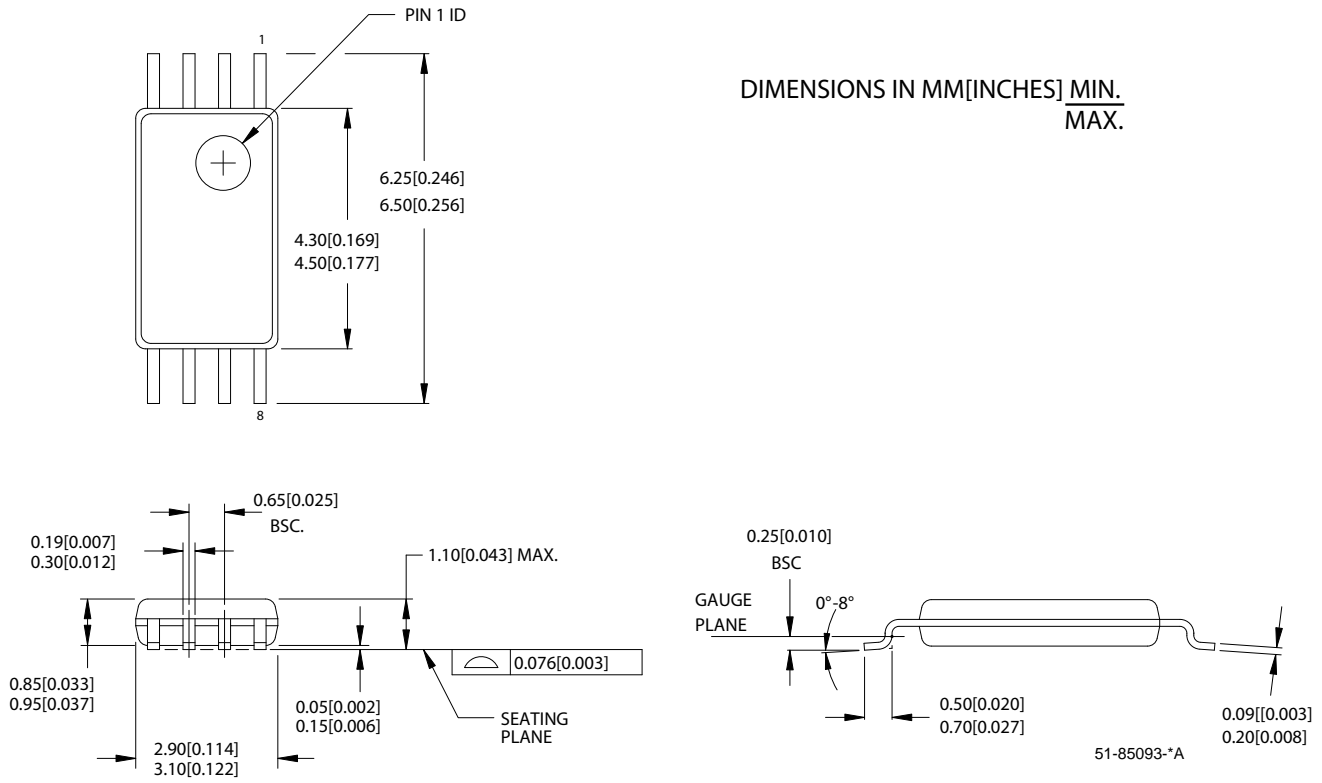
Figure 6. 8-Pin Thin Shrunk Small Outline Package (4.40 MM Body) Z8 (51-85093)
