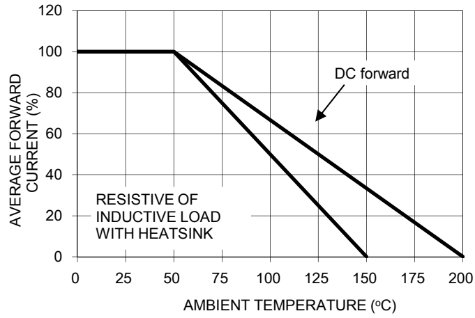
FIG.1 RATED FORWARD CURRENT VS AMBIENT TEMP. CURVE
