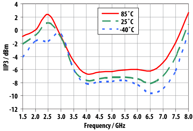
Figure 9. IIP3 vs Frequency
