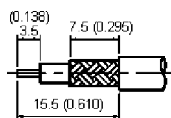
Stripping Dimension
