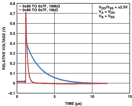
Figure 28. Maximum Transition Glitch
