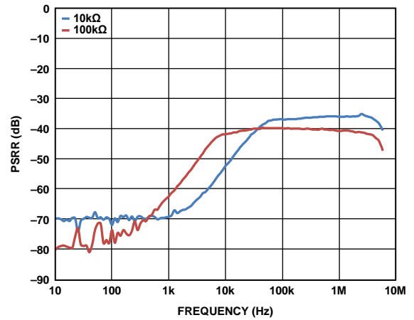
Figure 30. Power Supply Rejection Ratio (PSRR) vs. Frequency
