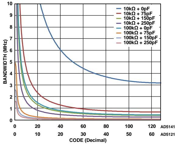
Figure 27. Maximum Bandwidth vs. Code vs. Net Capacitance
