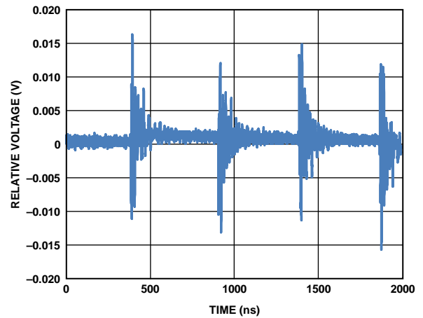
Figure 31. Digital Feedthrough
