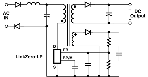
(a) Typical Application Schematic
