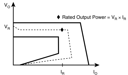
(b) Output Characteristic
