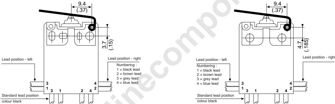
Actuators mounting position (type 139)
