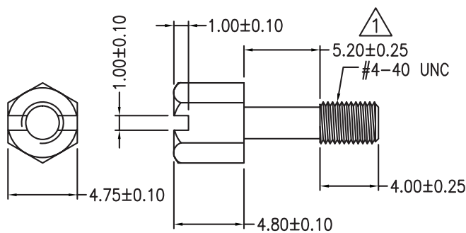
#4-40 UNC Hexscrew SCALE= 2.5:1
