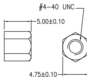
#4-40 UNC Hexnut SCALE= 2.5:1
