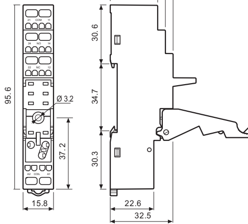
99.80 coil indication and EMC suppression modules for 95.55.3 socket
