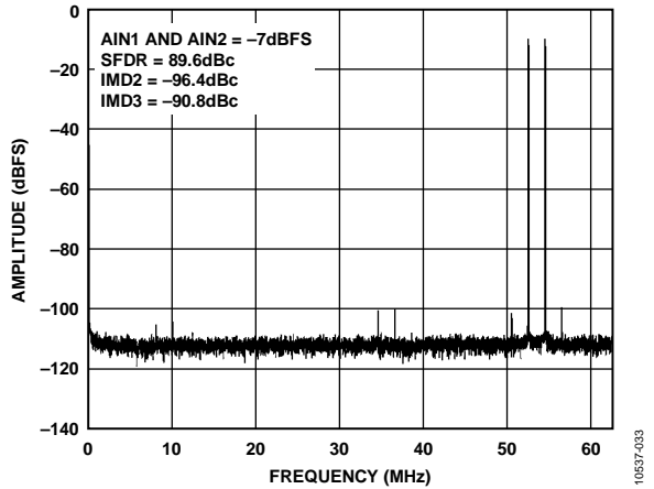
Figure 33. Two-Tone 16k FFT with f_{IN1} = 70.5 MHz and f_{IN2} = 72.5 MHz, f_{SAMPLE} = 125 MSPS
