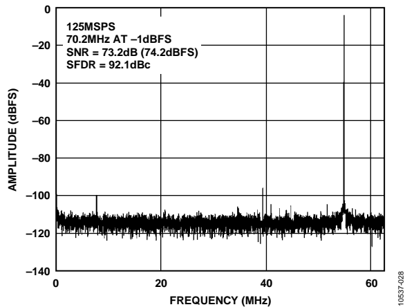
Figure 28. Single-Tone 16k FFT with f_{IN} = 70.2 MHz, f_{SAMPLE} = 125 MSPS
