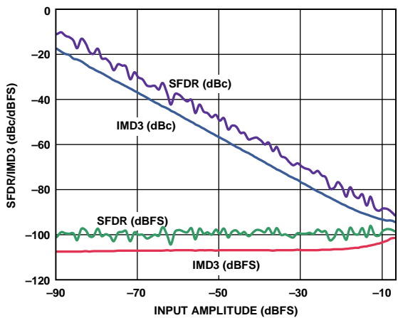
Figure 17. Two-Tone SFDR/IMD3 vs. Input Amplitude (AIN) with f_{IN1} = 70.5 MHz and f_{IN2} = 72.5 MHz, f_{SAMPLE} = 80 MSPS
