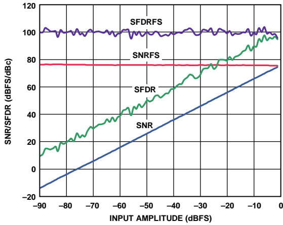
Figure 15. SNR/SFDR vs. Analog Input Level; f_{IN} = 9.7 MHz, f_{SAMPLE} = 80 MSPS
