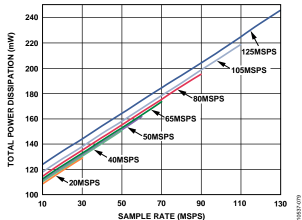
Figure 63. Total Power Dissipation vs. f_{SAMPLE} for f_{IN} = 9.7 \text{ MHz}
